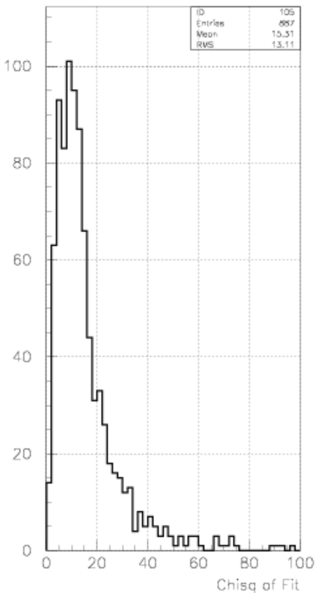
Least squares fit, Kpi2 decay, 6C fit ,cda, piomass
