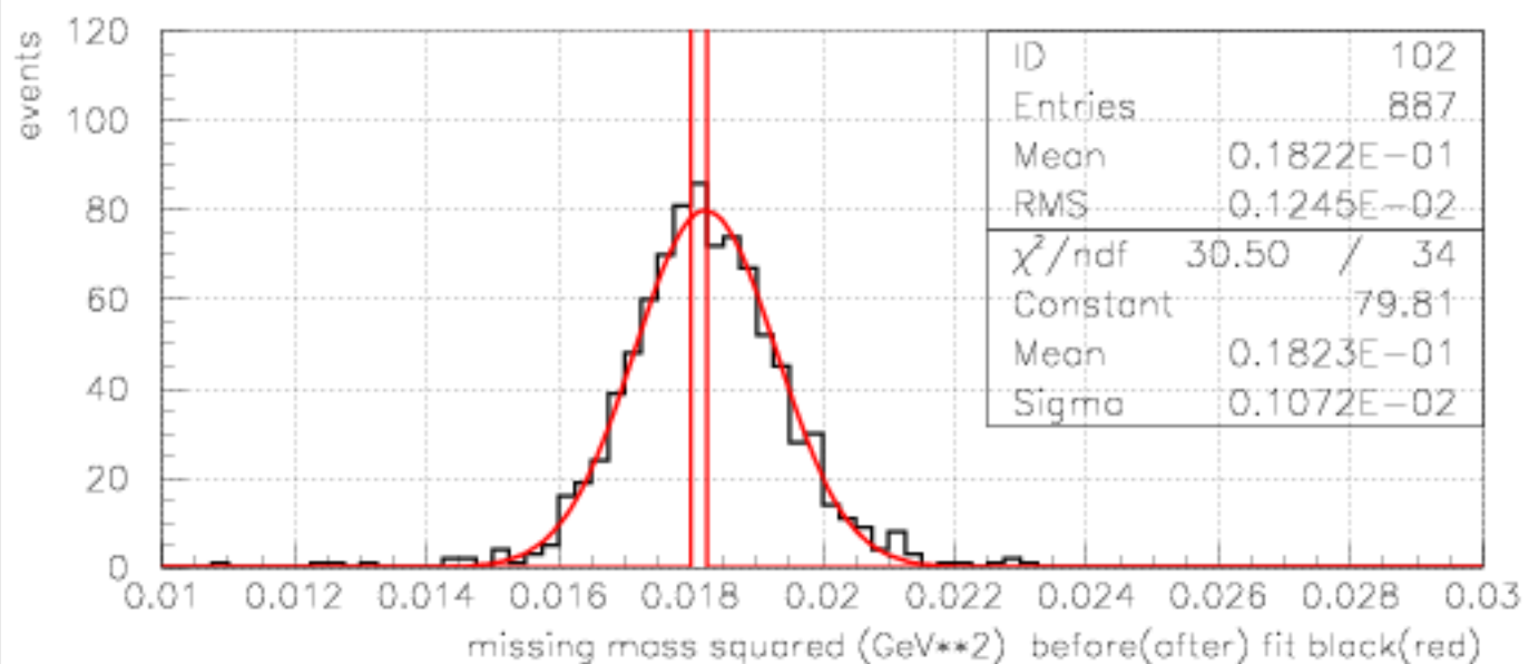
Least squares fit, Kpi2 decay, 6C fit ,cda, piomass
