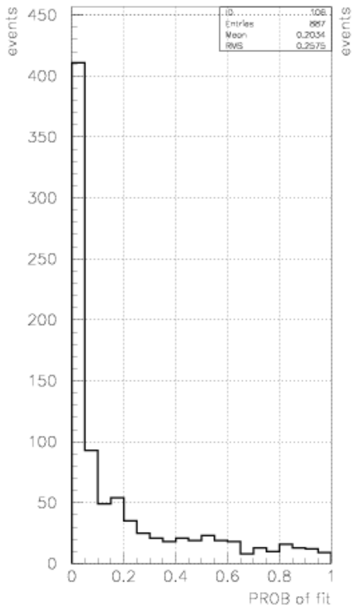
Least squares fit, Kpi2 decay, 6C fit ,cda, piomass
