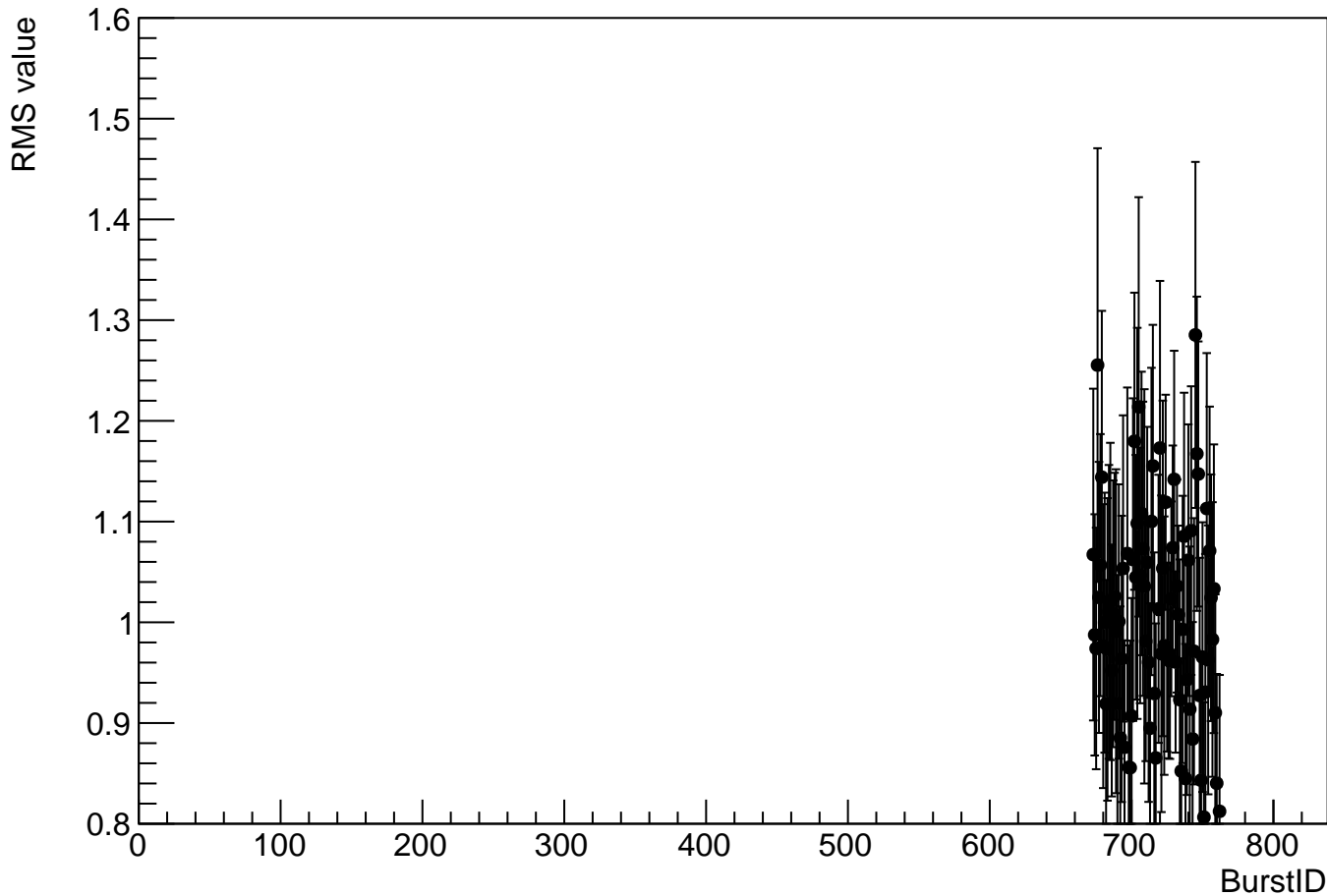
RMS_TimeWindow_-2.5ns_3.0ns_CHANITITimewrtTriggerTime
