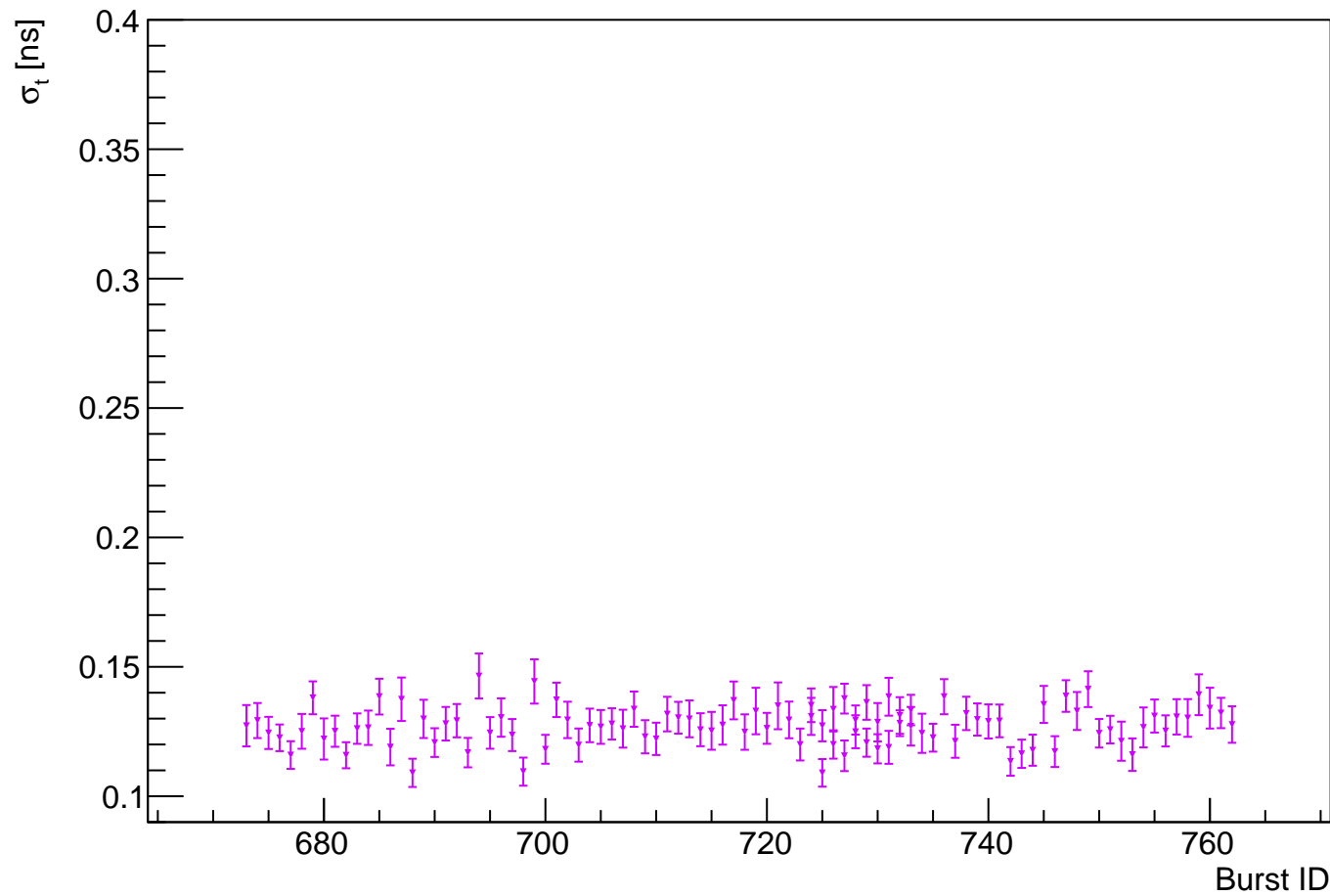
GTK-CEDAR time resolution vs BurstID for run 8094
