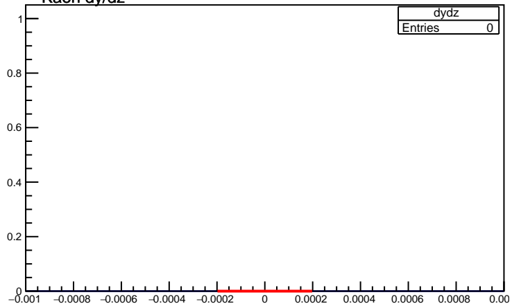
Kaon dy/dz
