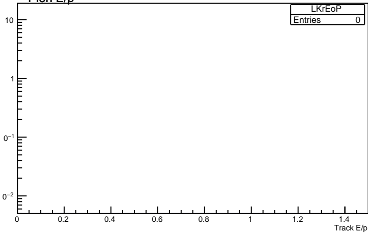
Pion E/p
