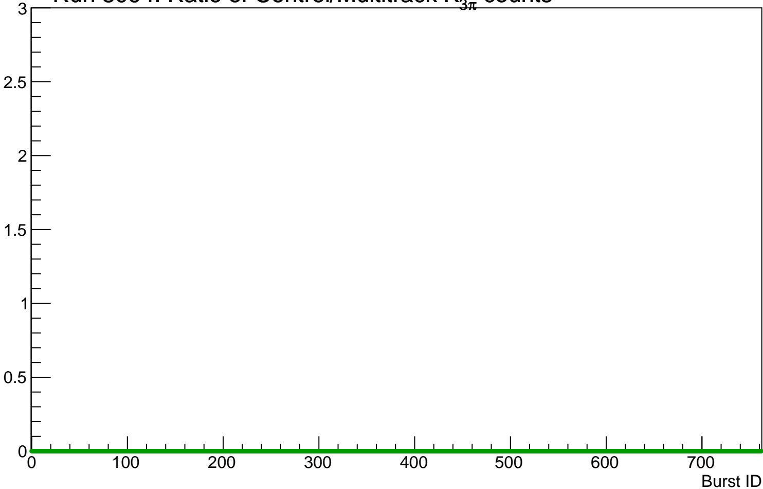
Run 8094: Ratio of Control/Multitrack K_{3\pi} counts
