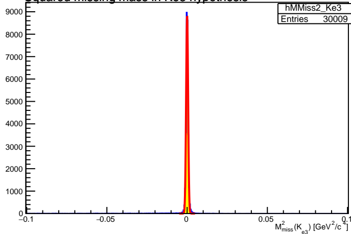
Squared missing mass in Ke3 hypothesis
