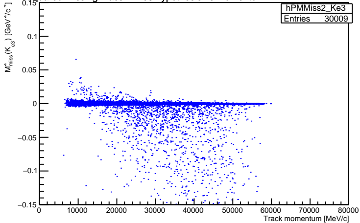
Squared missing mass in Ke3 hypothesis vs momentum
