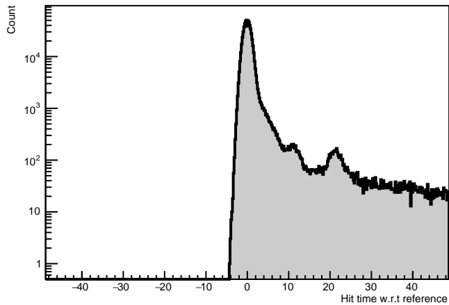
DigiTimeRaw_Phys1I_NewCHOD
