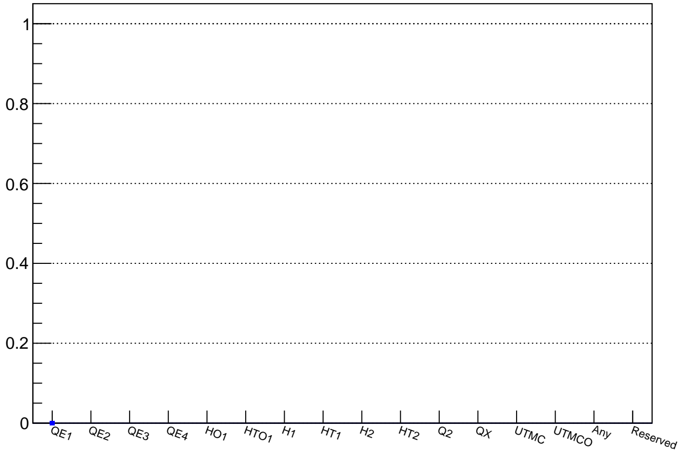
NewCHOD trigger probability for K3pi_UTMC candidates (0 events)
