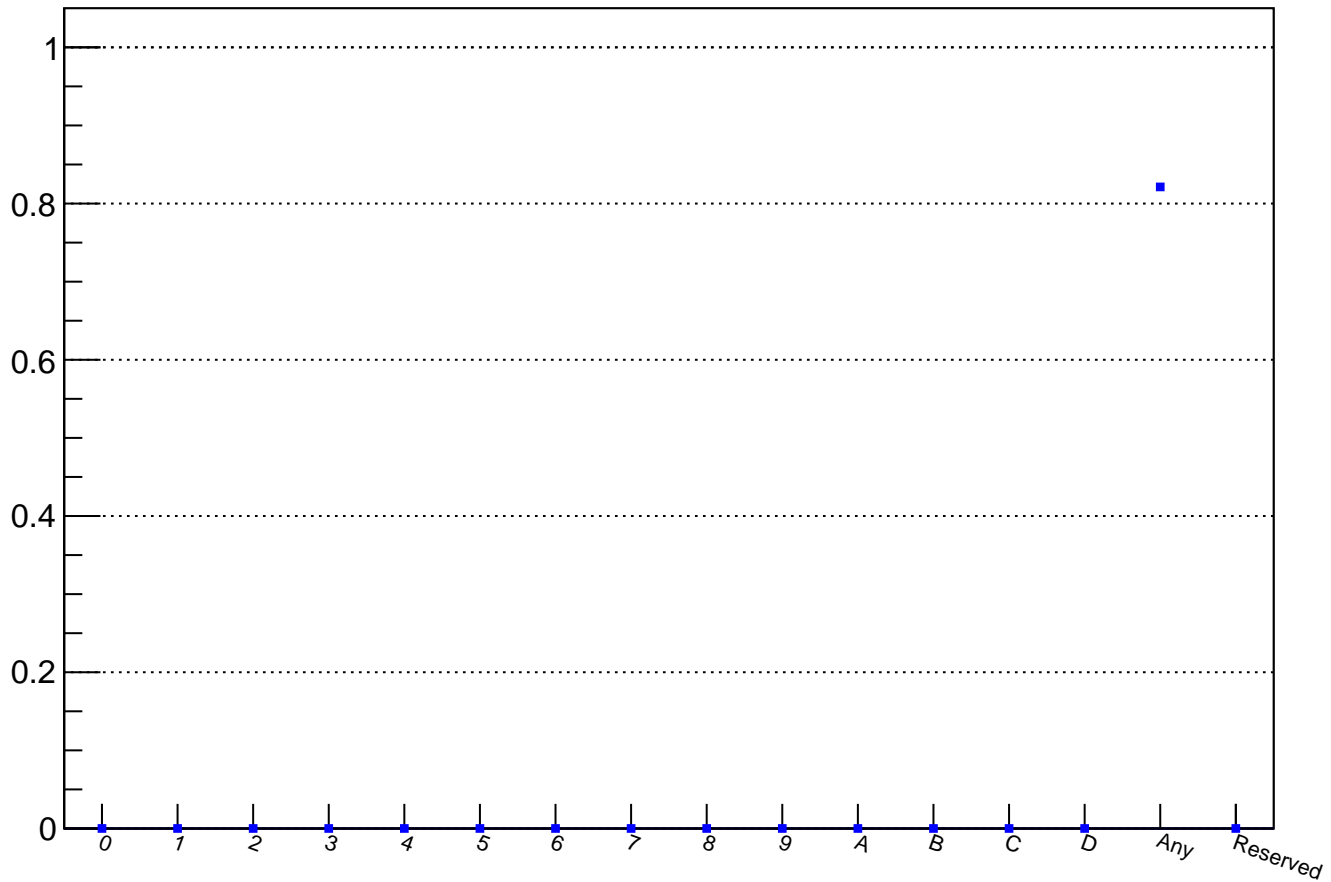
Calo trigger probability for Mask10 candidates (193842 events)
