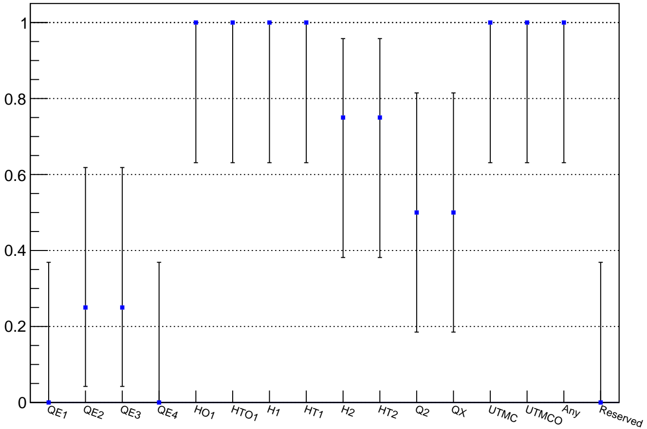
NewCHOD trigger probability for Kmu2_M1 candidates (4 events)
