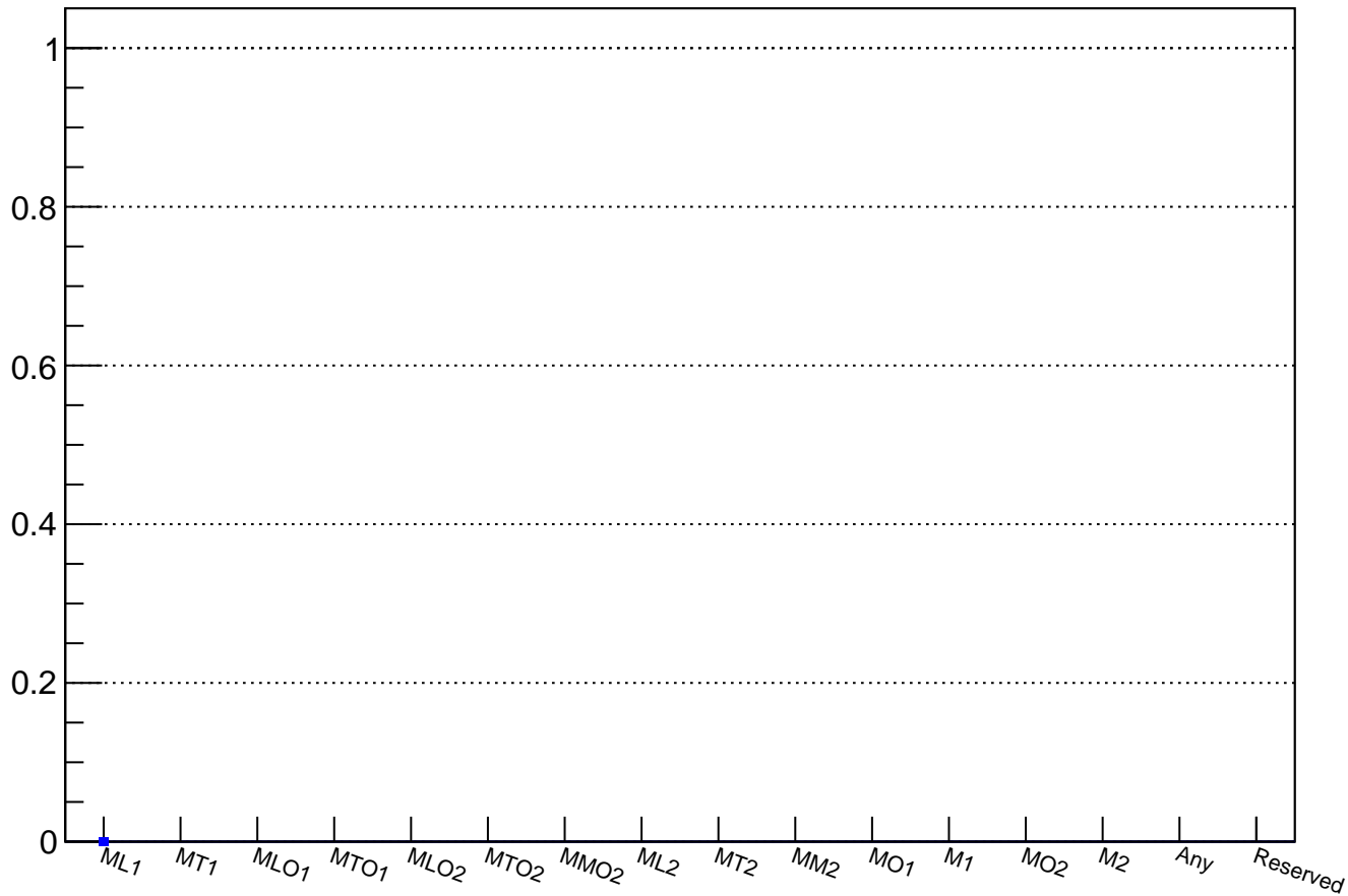
MUV3 trigger probability for K3pi_Q2 candidates (0 events)
