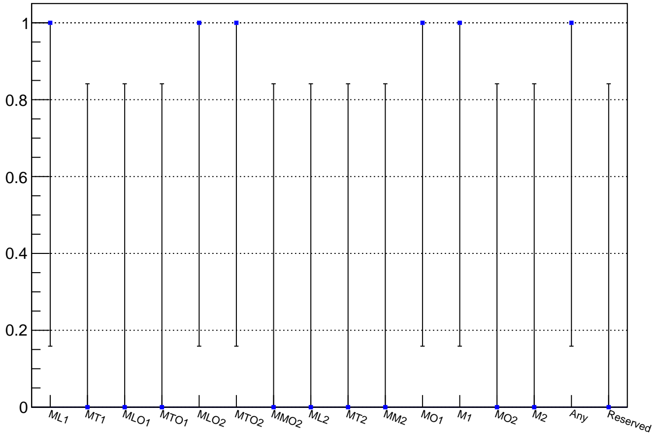
MUV3 trigger probability for Kmu2_MO2 candidates (1 events)
