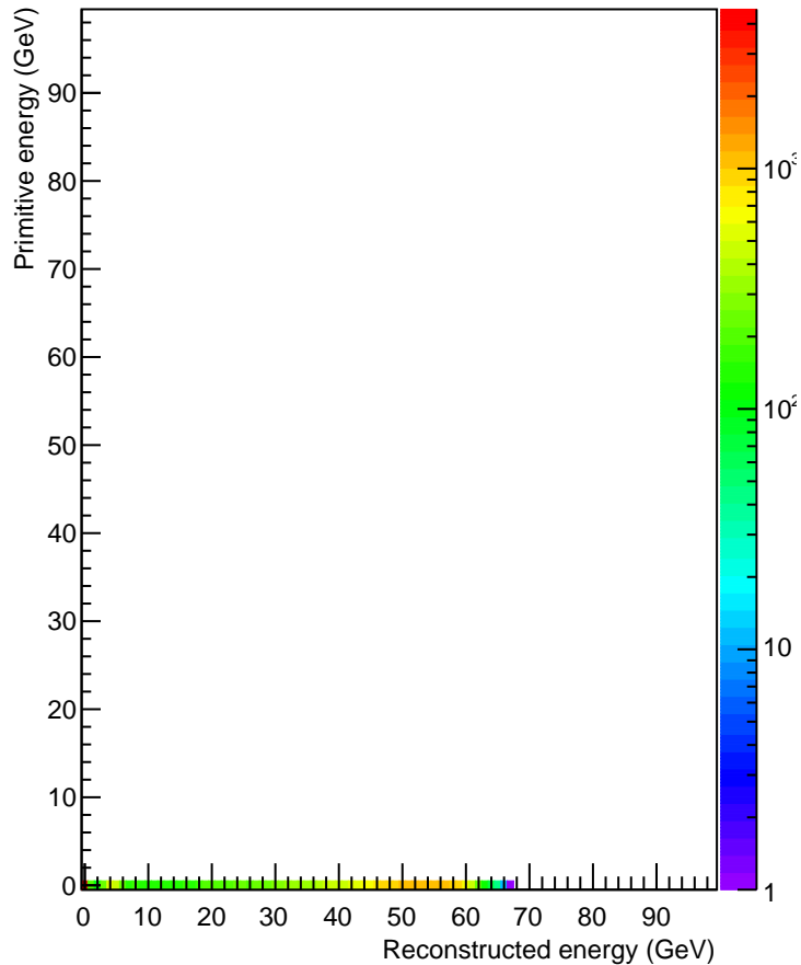
LKrEnergy2D
