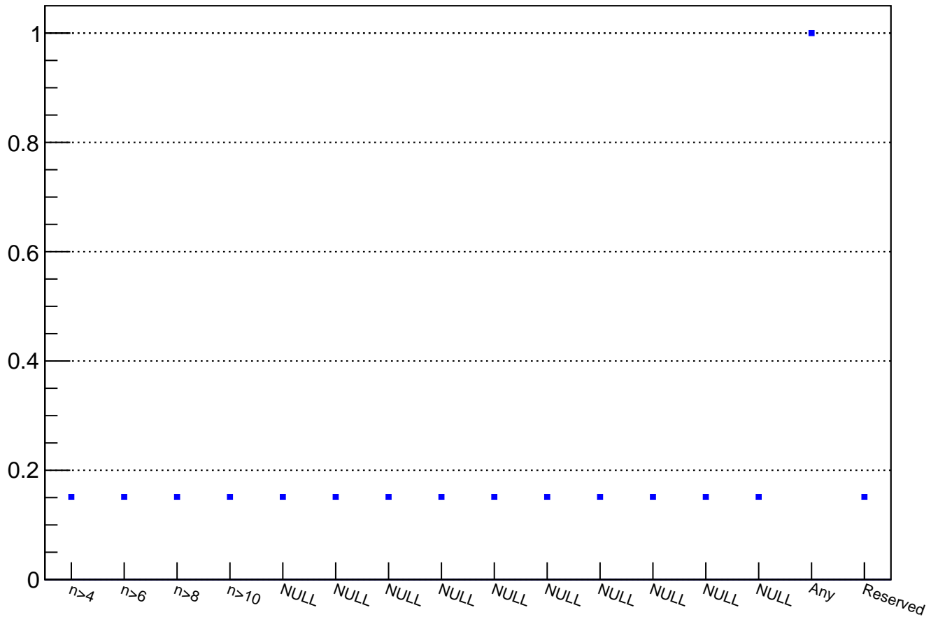
RICH trigger probability for Mask5 candidates (193842 events)
