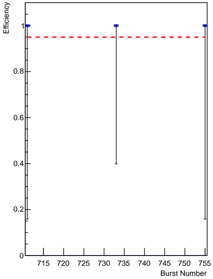
R2 efficiency per burst (Kmu2 events)
