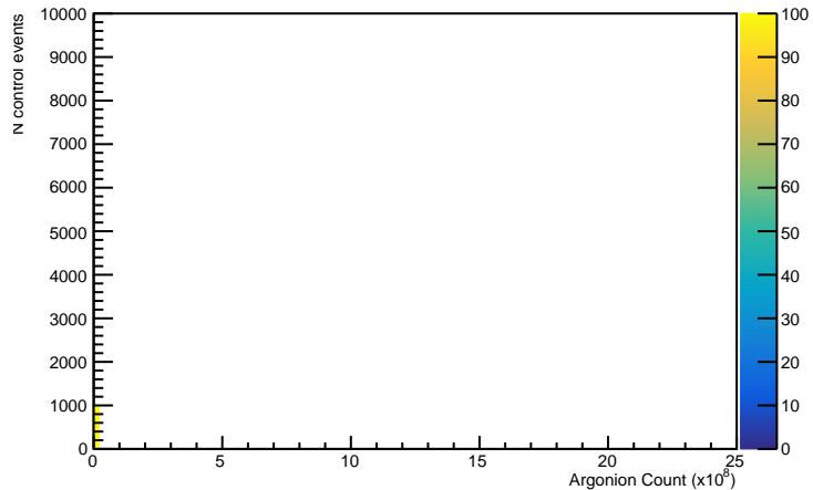
ControlVsArgonion
