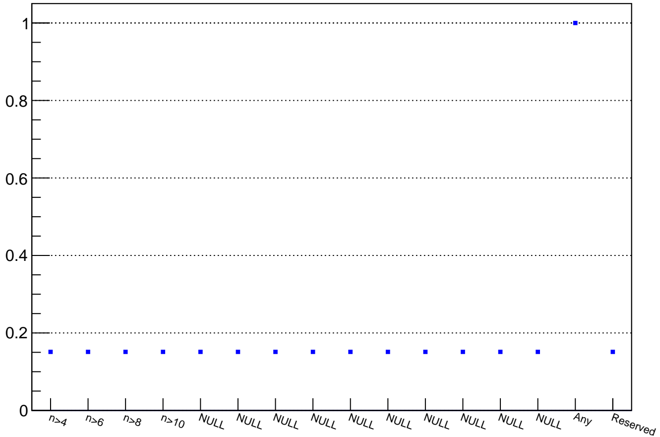
RICH trigger probability for Mask6 candidates (193842 events)
