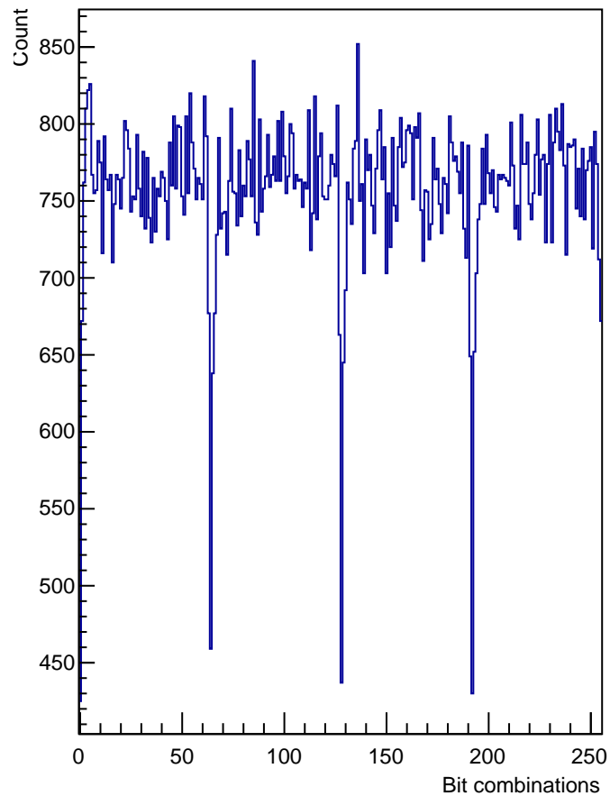
PrimitiveFTBits_RICH_RICH
