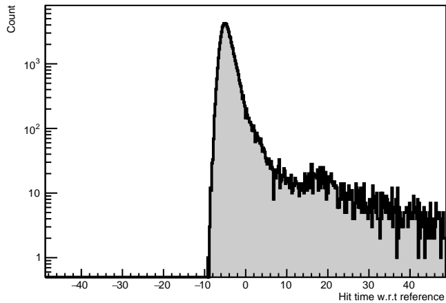
DigiTimeRaw_Control_NewCHOD
