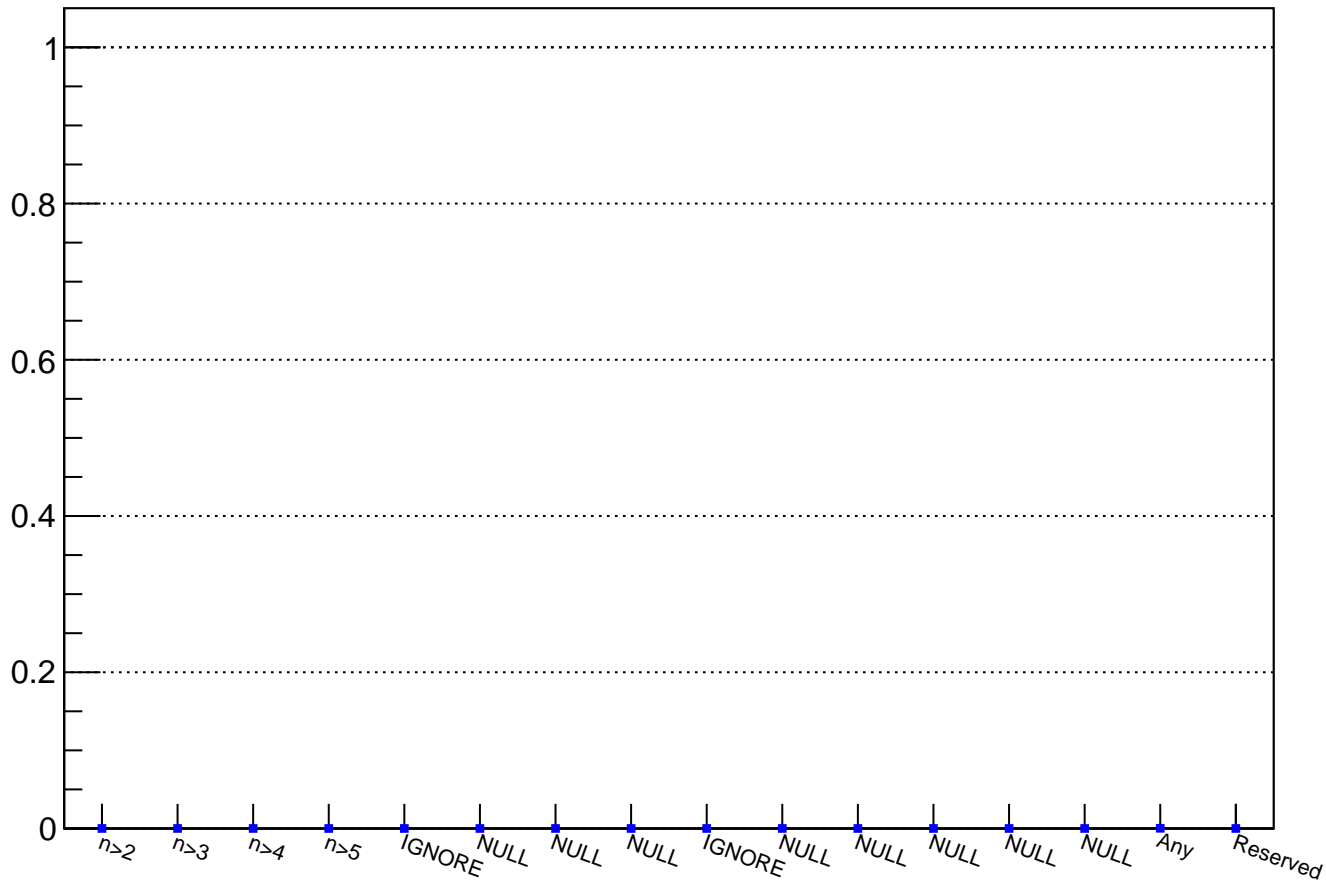
LAV12 trigger probability for K2pi candidates (3921 events)
