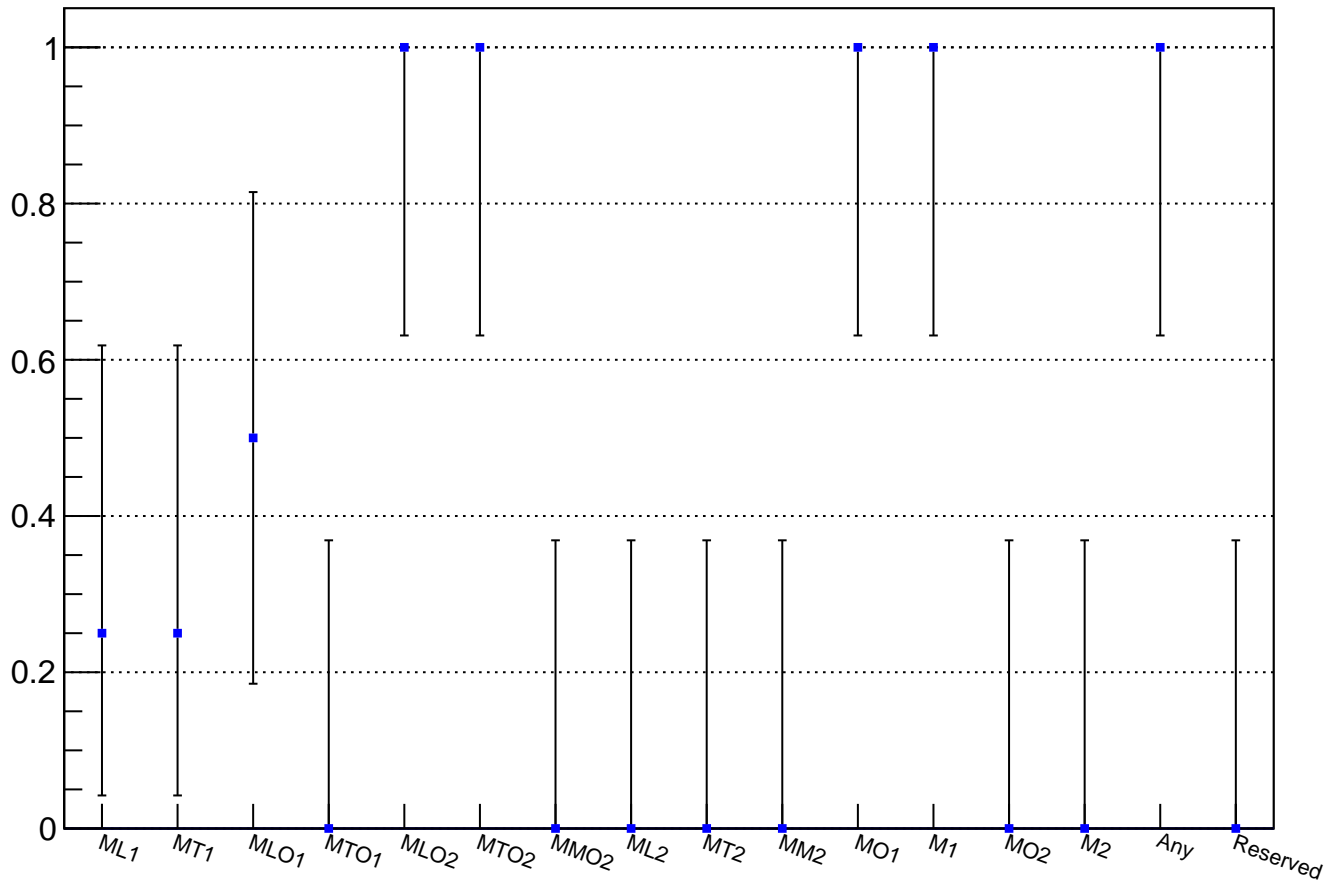
MUV3 trigger probability for Kmu2_UTMC candidates (4 events)
