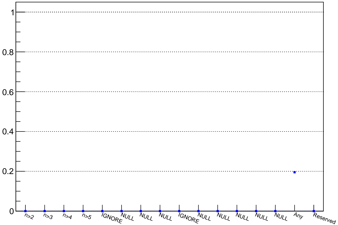
LAV12 trigger probability for Mask0 candidates (193842 events)
