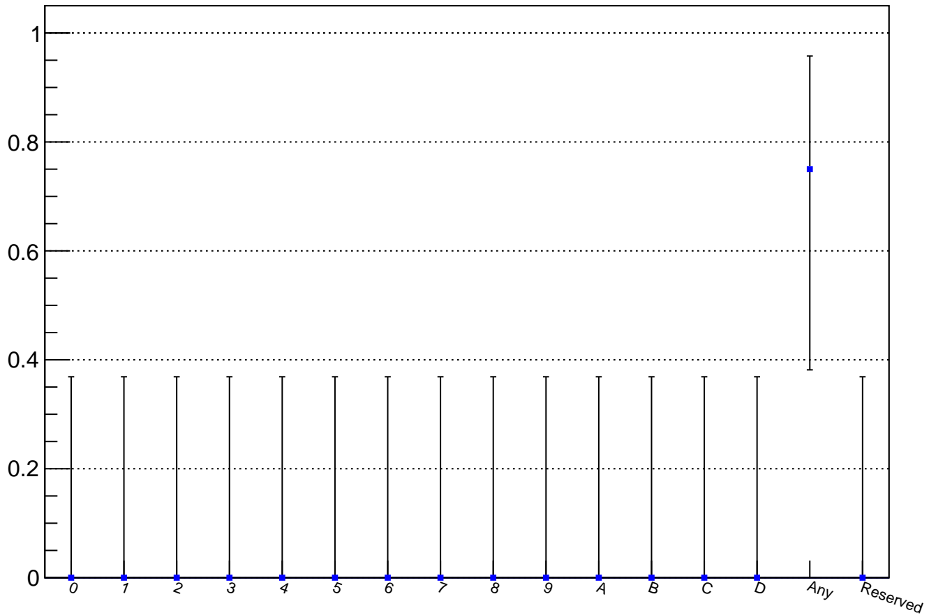
Calo trigger probability for Kmu2_UTMC candidates (4 events)
