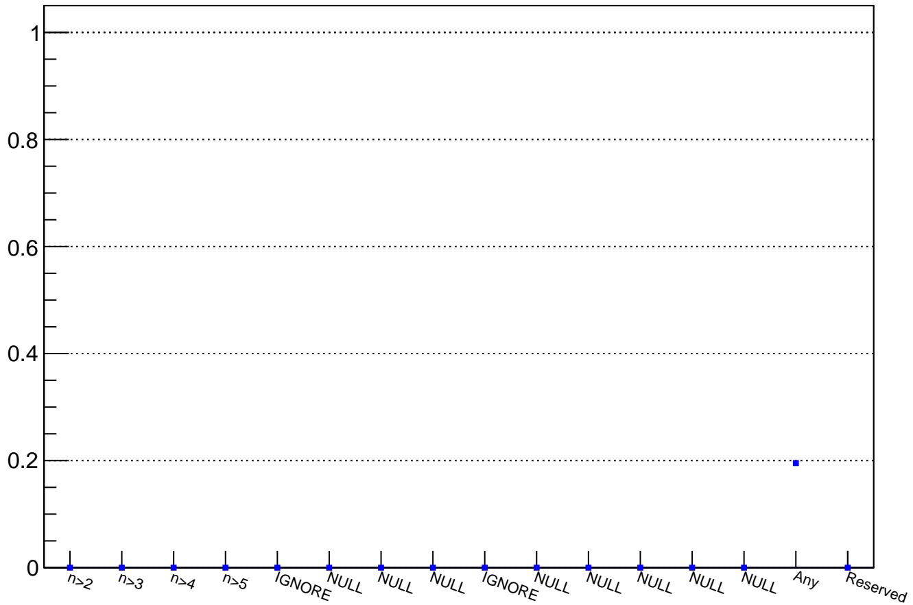
LAV12 trigger probability for Mask15 candidates (193842 events)
