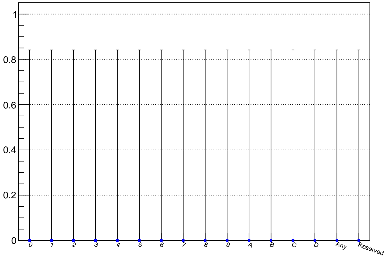
Calo trigger probability for Kmu2_MO2 candidates (1 events)
