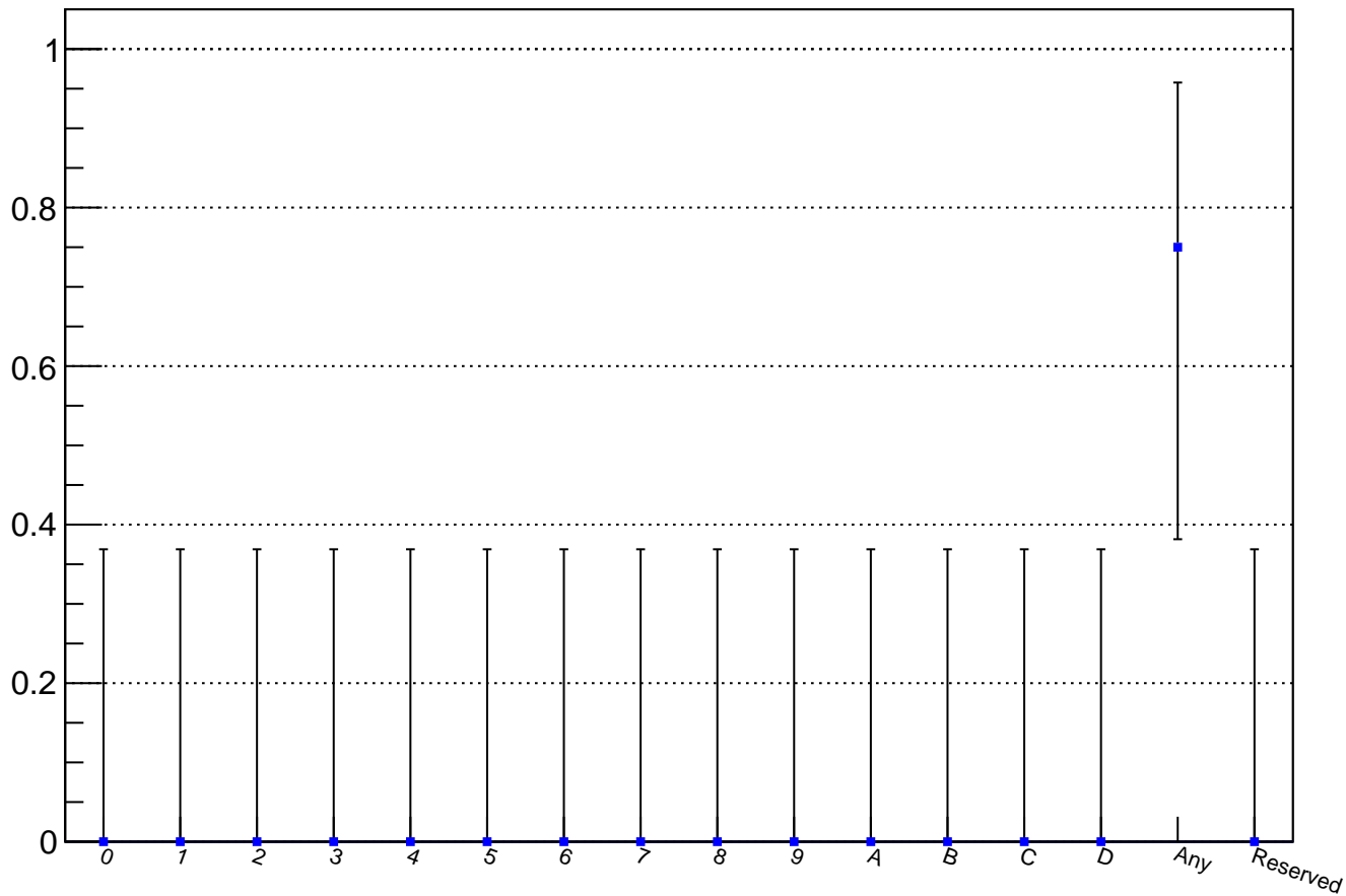
Calo trigger probability for Kmu2_M1 candidates (4 events)
