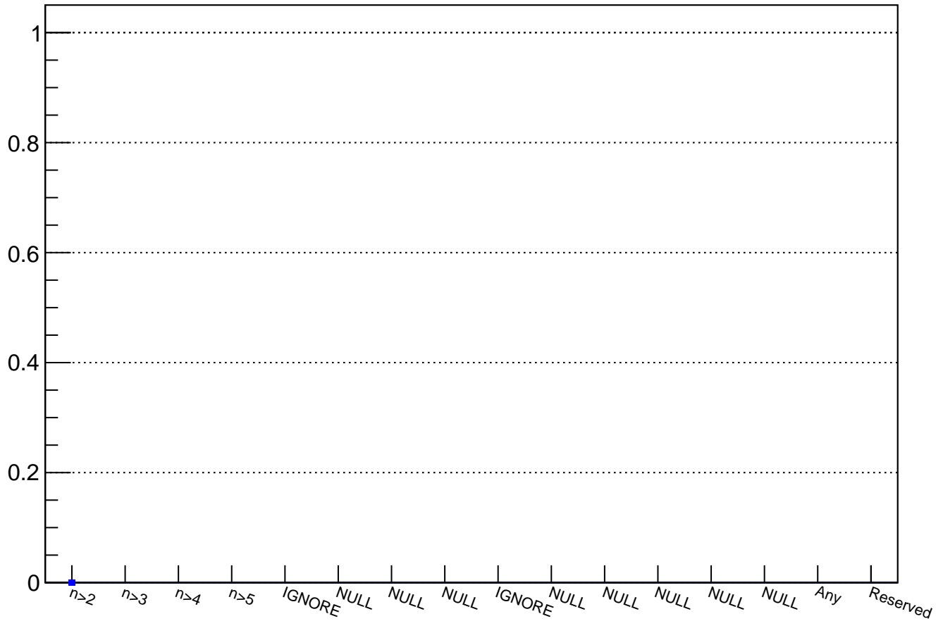
LAV12 trigger probability for K3pi_QX3H candidates (0 events)
