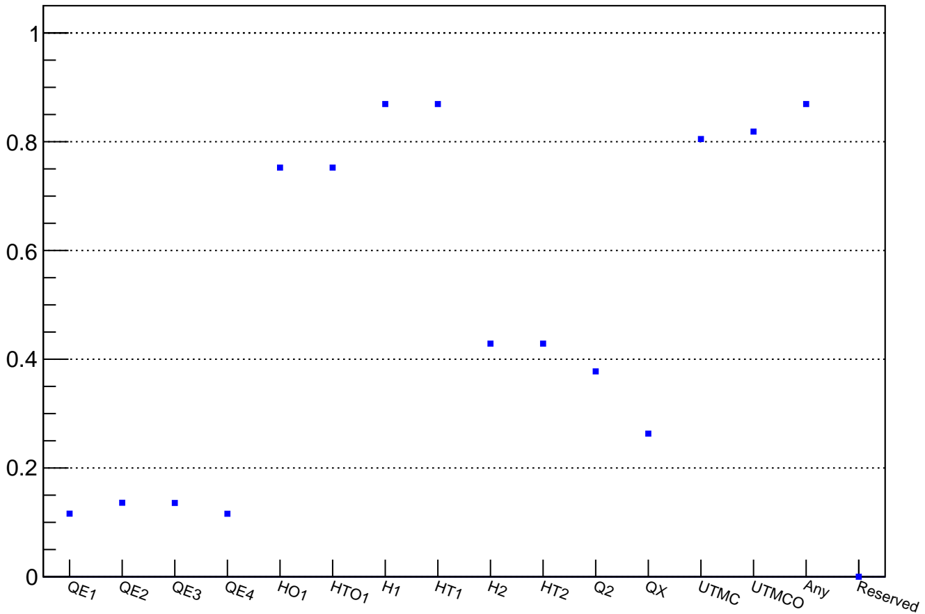
NewCHOD trigger probability for Mask0 candidates (193842 events)
