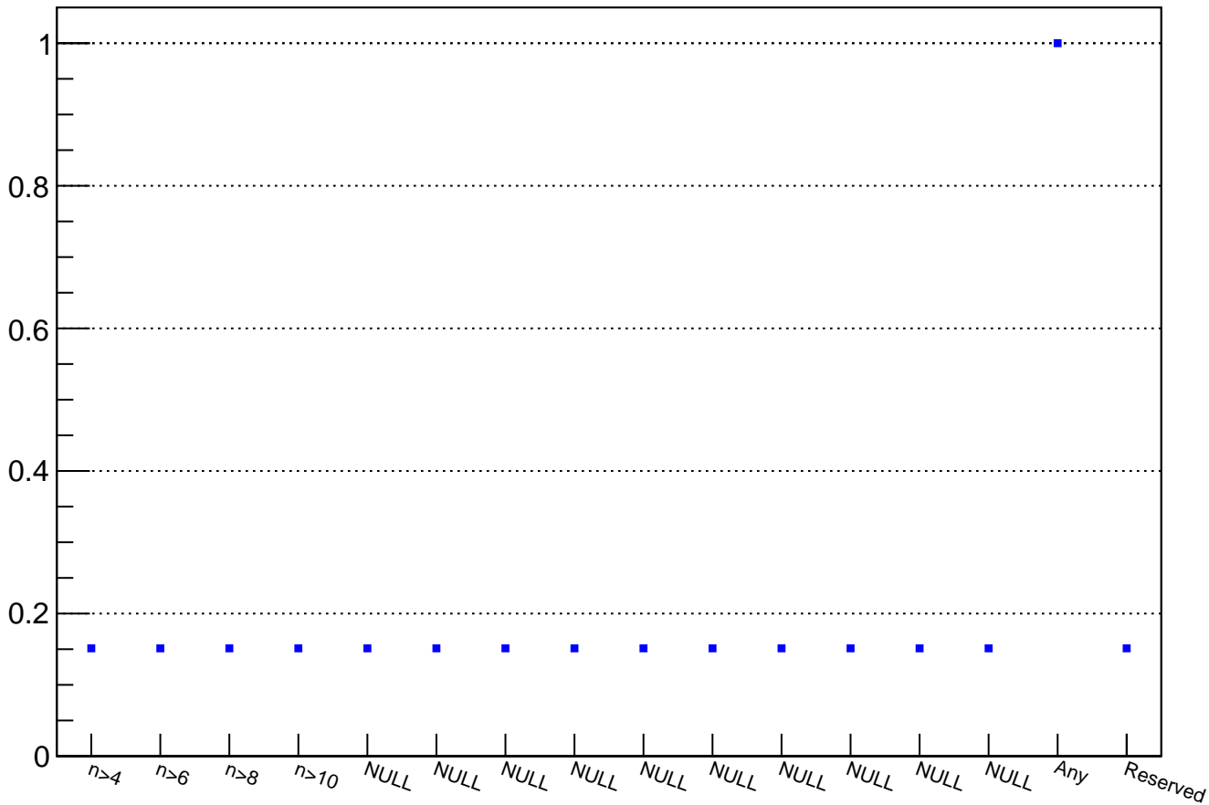
RICH trigger probability for Mask11 candidates (193842 events)
