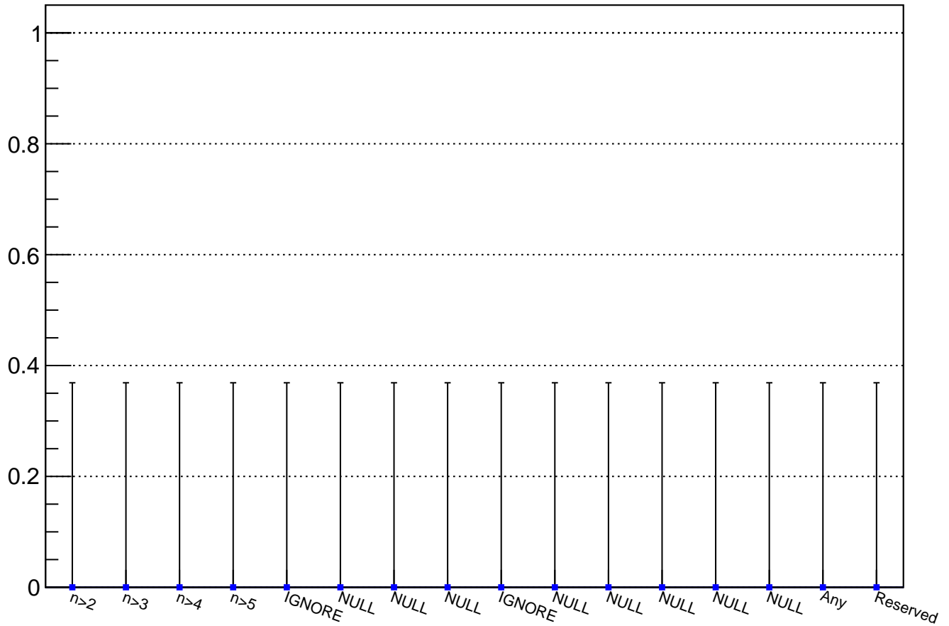
LAV12 trigger probability for Kmu2_M1 candidates (4 events)
