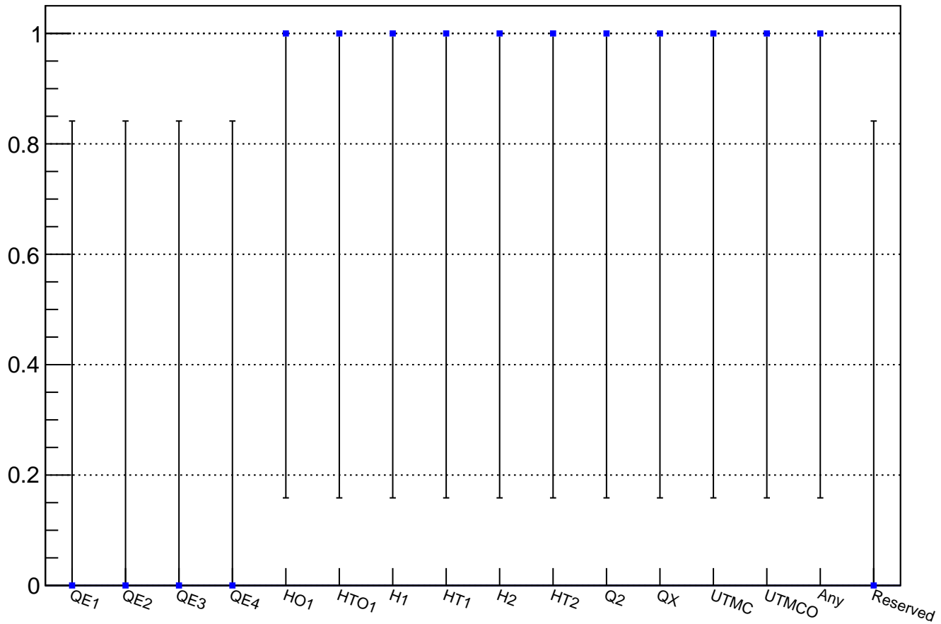
NewCHOD trigger probability for Kmu2_M2 candidates (1 events)
