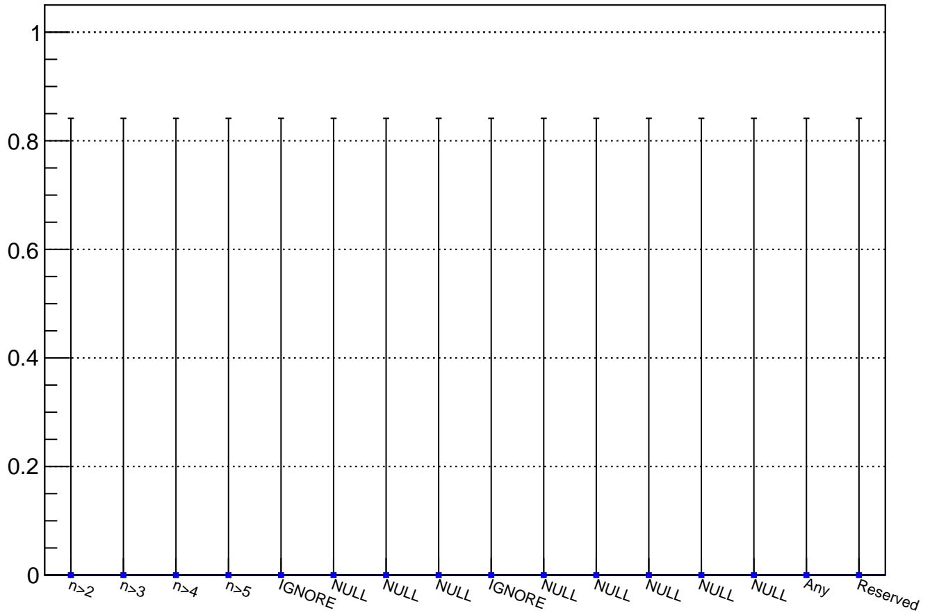
LAV12 trigger probability for Kmu2_MO2 candidates (1 events)
