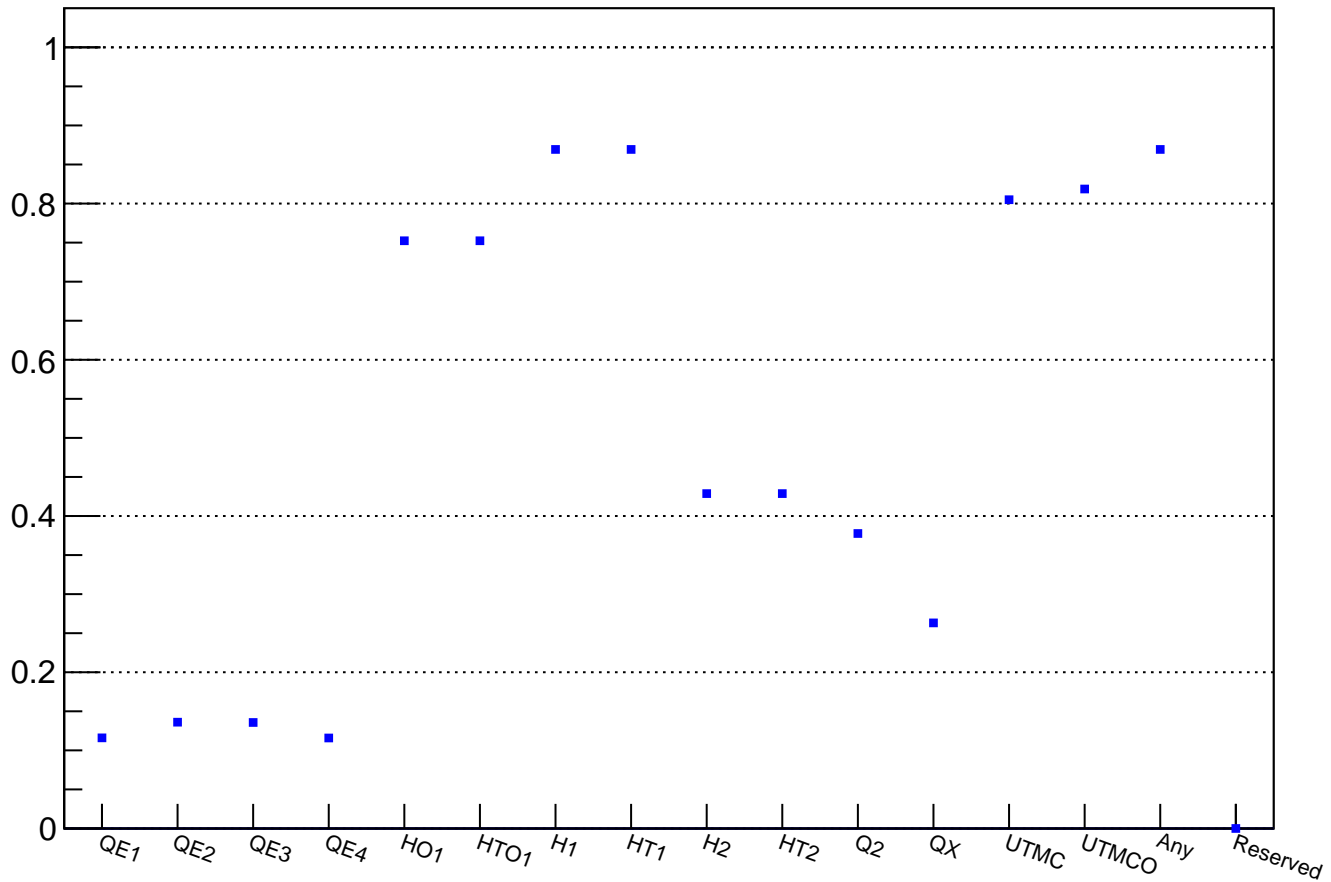
NewCHOD trigger probability for Mask12 candidates (193842 events)
