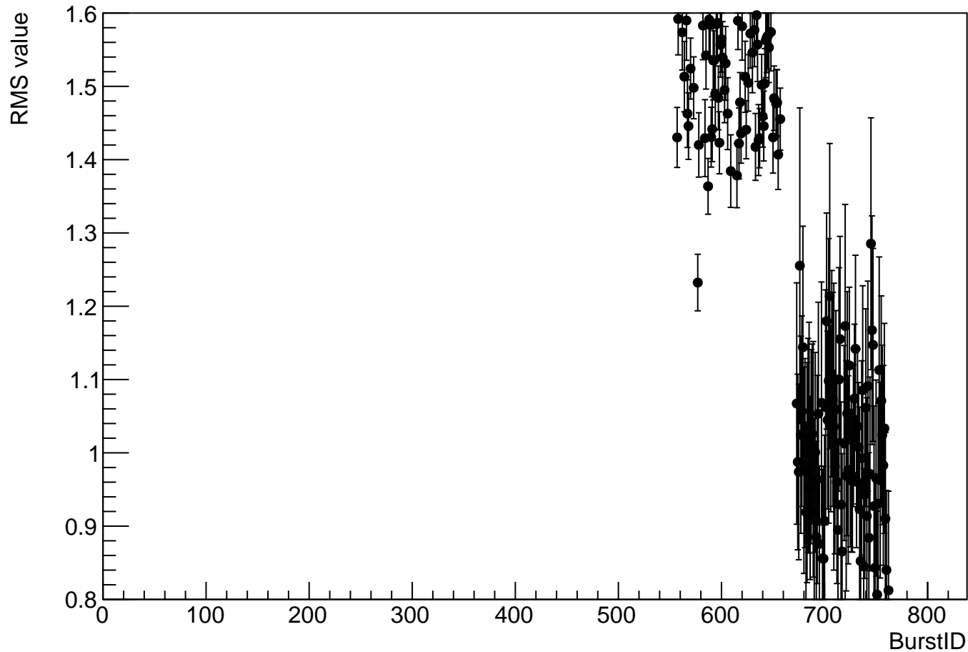
RMS_TimeWindow_-2.5ns_3.0ns_CHANIT1TimewrtTriggerTime
