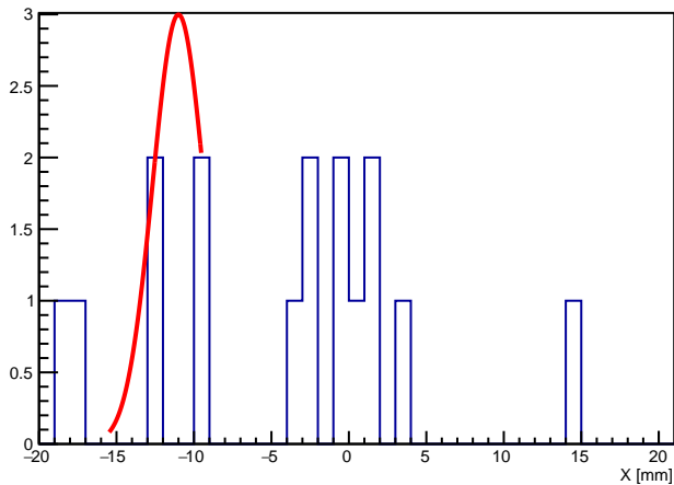
Track extrapolation to the CHOD H plane, no hits in CHOD H
