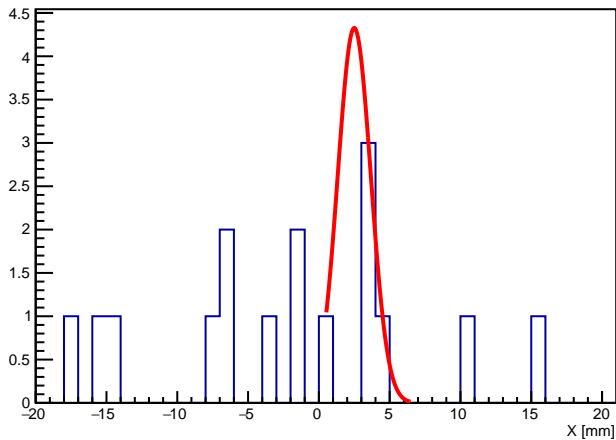
Track extrapolation to the CHOD V plane, no hits in CHOD V
