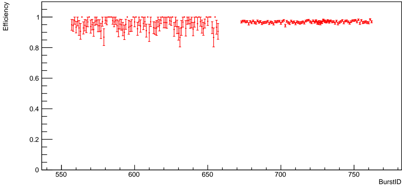
efficiency Vs BurstID for run 8094 (single track, no shower)
