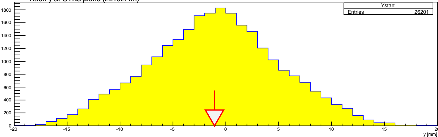
Kaon y at GTK3 plane (z=102.4m)
