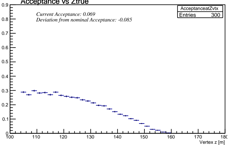
Acceptance vs Ztrue
