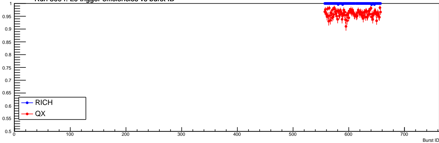
Run 8094: L1 trigger efficiencies vs burst ID
