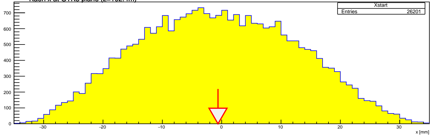
Kaon x at GTK3 plane (z=102.4m)
