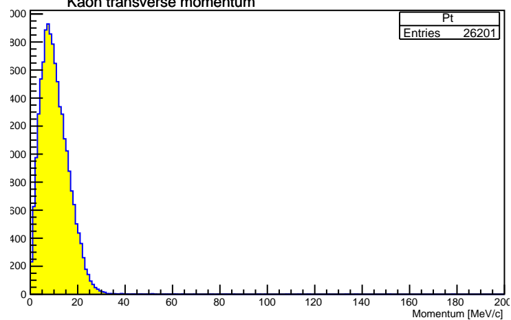
Kaon transverse momentum
