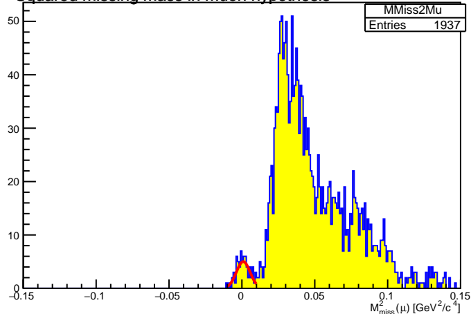
Squared missing mass in muon hypothesis
