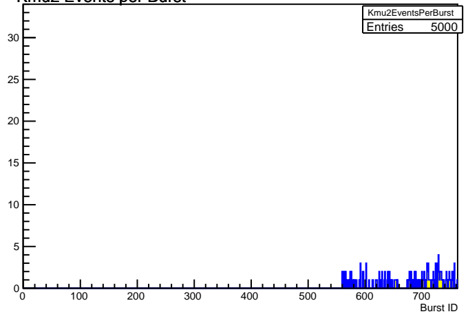
Kmu2 Events per Burst
