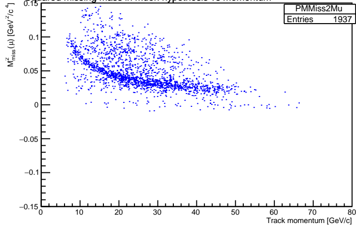
Squared missing mass in muon hypothesis vs momentum
