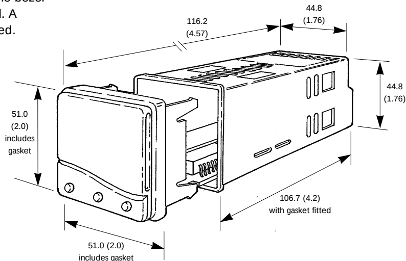
Model 9300 Dimensions in mm (inches)
