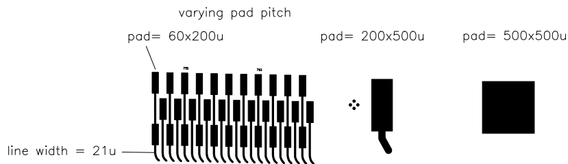
DETECTOR SIDE CORNER DETAIL
