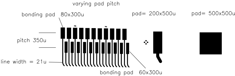
DETECTOR SIDE CORNER DETAIL
