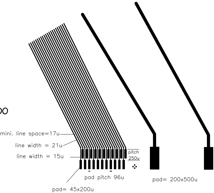
CHIP SIDE CORNER DETAIL
