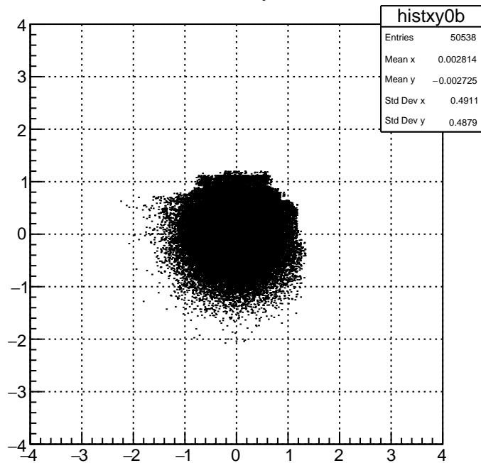
BDT histxy0b
