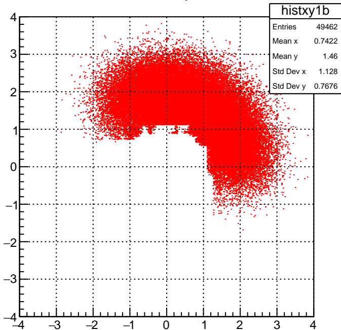
BDT histxy1b
