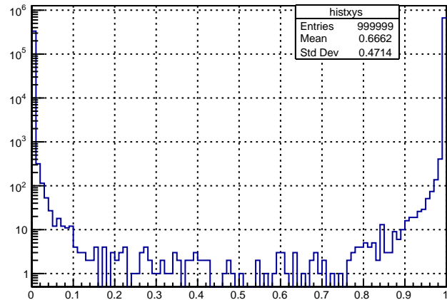
MLP Response
