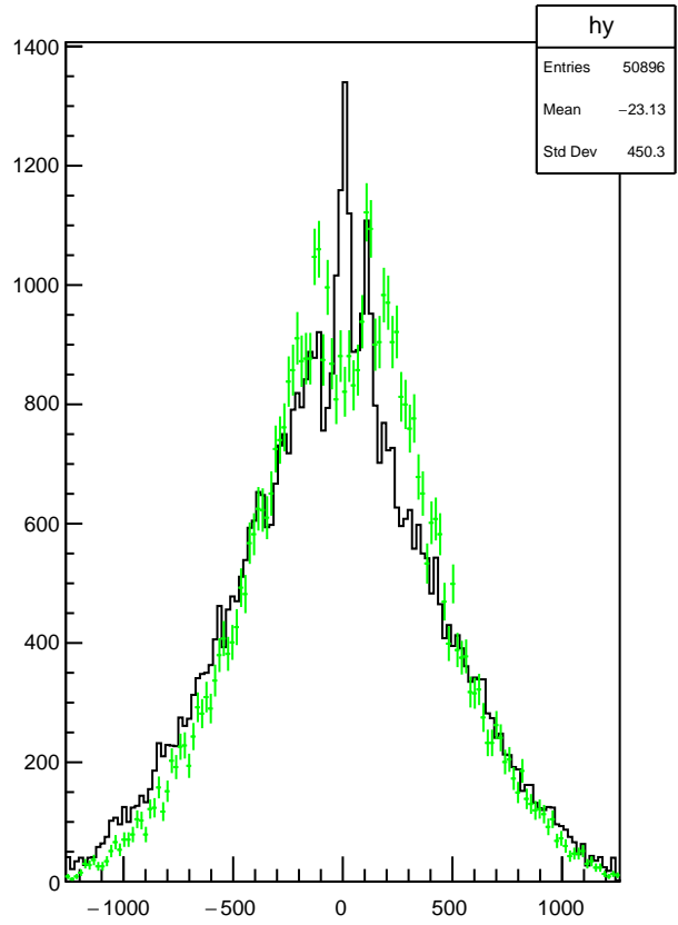
Plot 6 TwoPhotonAnalysis/MipClusterXY 29
