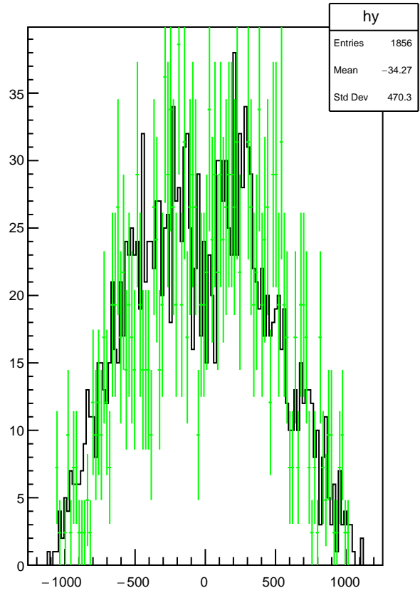
Plot 11 TwoPhotonAnalysis/EMClusterXY_low_pnn 35
