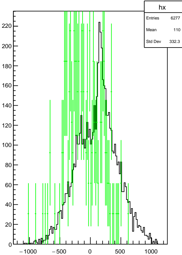
Plot 10 TwoPhotonAnalysis/EMClusterXY_high_ctr 34
