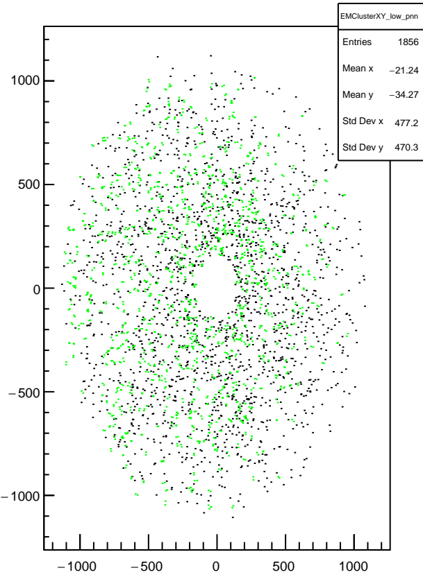
Plot 11 TwoPhotonAnalysis/EMClusterXY_low_pnn 35
