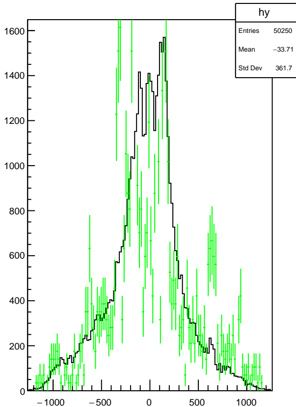
Plot 13 TwoPhotonAnalysis/OtherClusterXY 38
