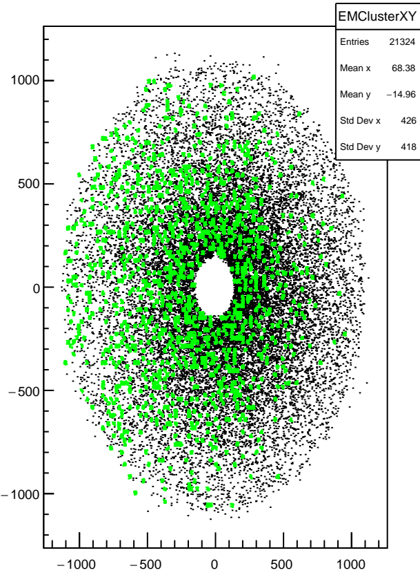
Plot 8 TwoPhotonAnalysis/EMClusterXY
