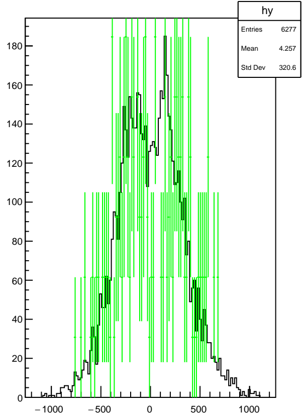
Plot 10 TwoPhotonAnalysis/EMClusterXY_high_ctr 34
