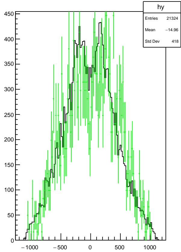
Plot 8 TwoPhotonAnalysis/EMClusterXY
