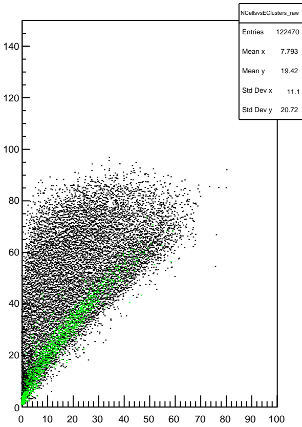
Plot 4 TwoPhotonAnalysis/NCellsvsEClusters_raw 25
