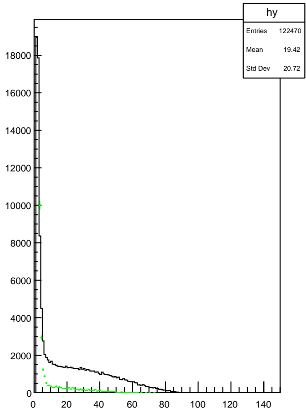
Plot 4 TwoPhotonAnalysis/NCellsvsEClusters_raw 25
