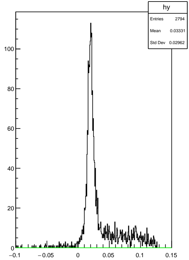
Plot 2 TwoPhotonAnalysis/Pi0_mmissVSPHi_pic 7
