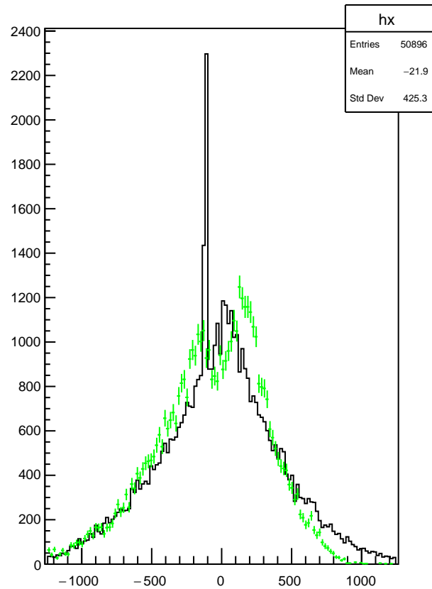
Plot 6 TwoPhotonAnalysis/MipClusterXY 29
