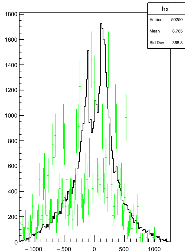
Plot 13 TwoPhotonAnalysis/OtherClusterXY 38
