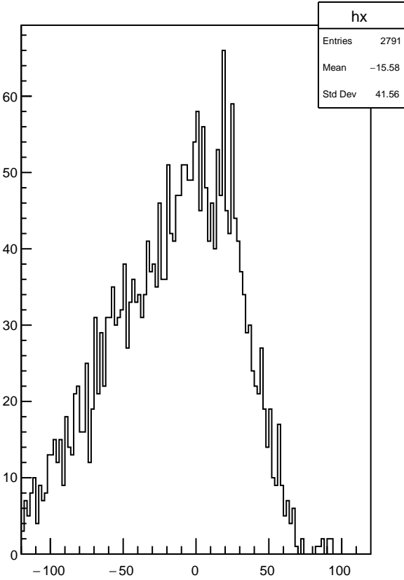
Plot 1 TwoPhotonAnalysis/Pic_posAtCHOD 5
