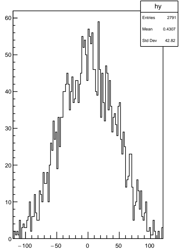
Plot 1 TwoPhotonAnalysis/Pic_posAtCHOD 5
