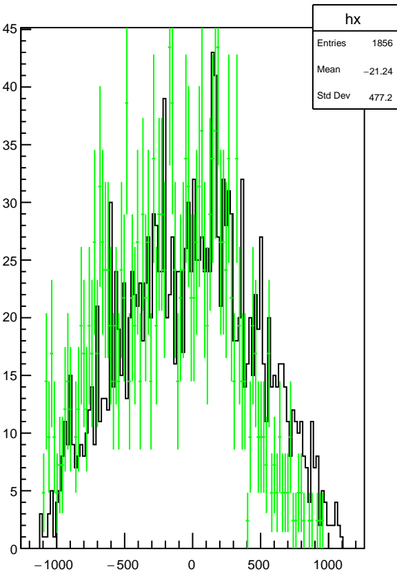
Plot 11 TwoPhotonAnalysis/EMClusterXY_low_pnn 35
