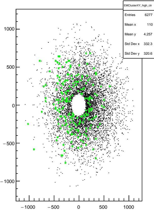
Plot 10 TwoPhotonAnalysis/EMClusterXY_high_ctr 34
