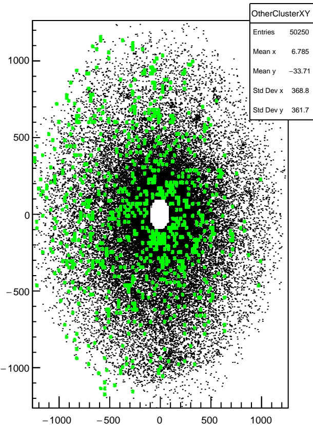
Plot 13 TwoPhotonAnalysis/OtherClusterXY 38
