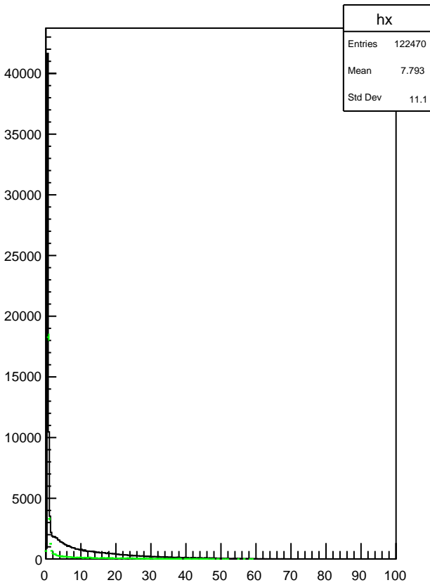
Plot 4 TwoPhotonAnalysis/NCellsvsEClusters_raw 25
