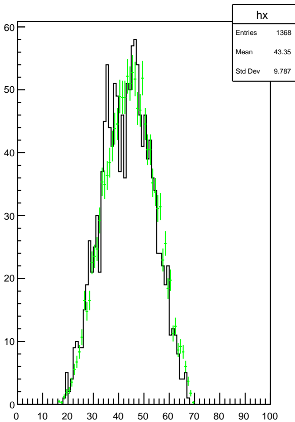
Plot 4 TwoPhotonAnalysis/Pi0_mmiss 9
