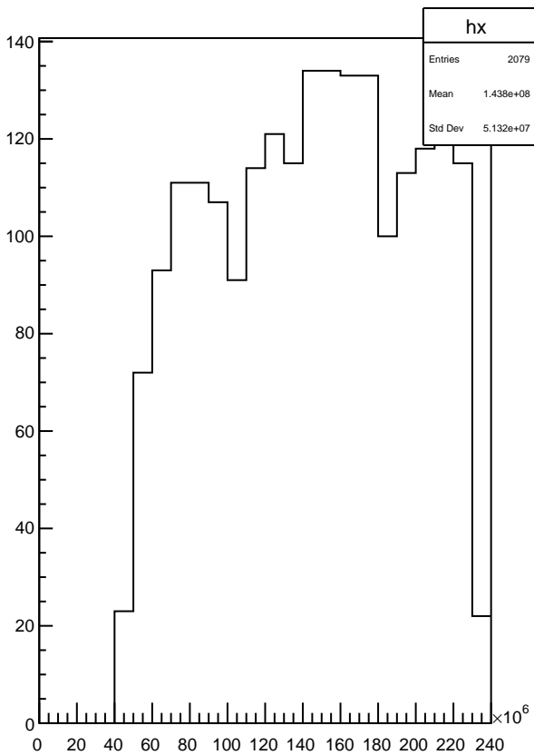
Plot 7 TwoPhotonAnalysis/Pi0_mmiss_timestamp 13
