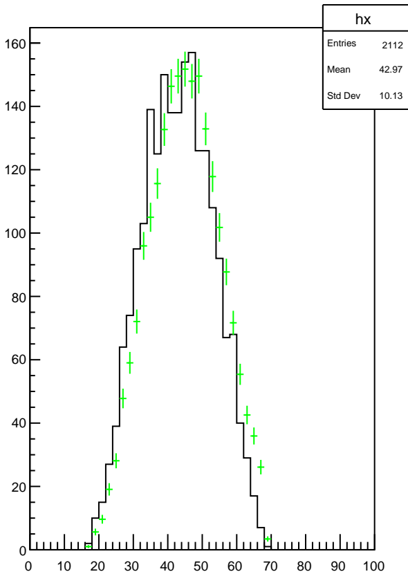
Plot 5 TwoPhotonAnalysis/Pi0_mmiss_acceptance 11
