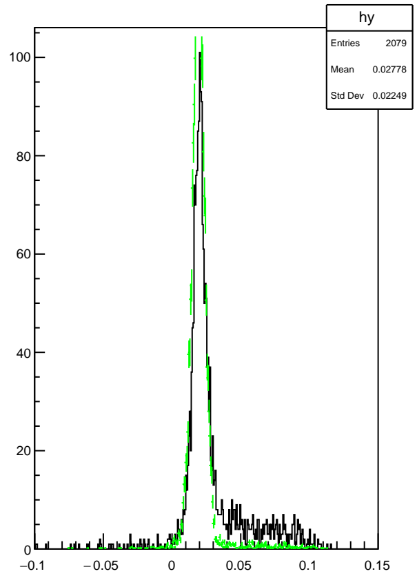
Plot 6 TwoPhotonAnalysis/Pi0_mmiss_isolation 12
