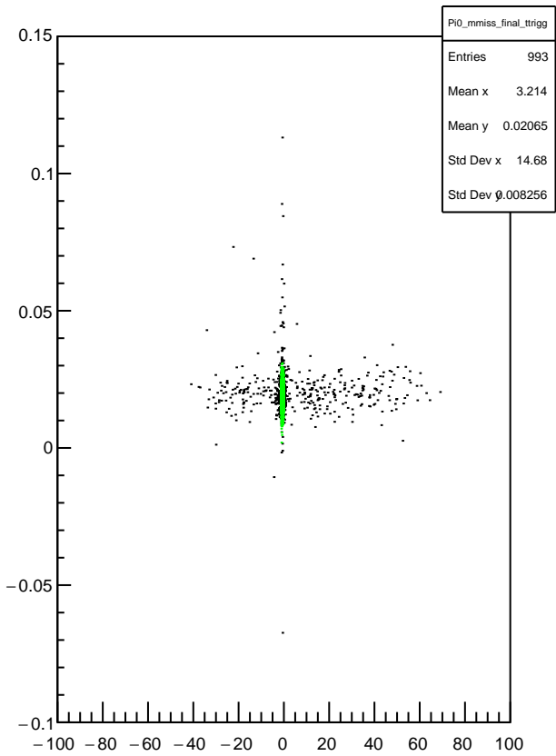
Plot 15 TwoPhotonAnalysis/Pi0_mmiss_final_trigg 21
