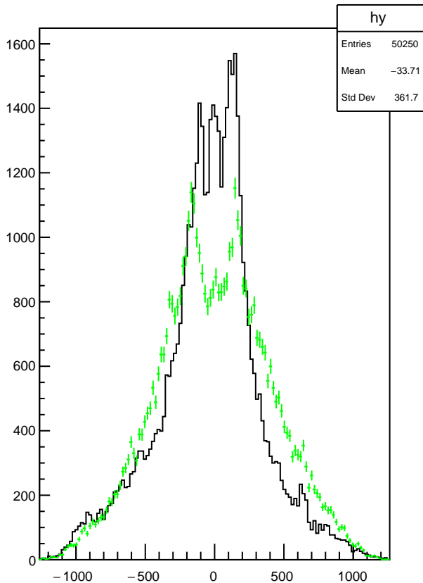
Plot 25 TwoPhotonAnalysis/OtherClusterXY 38
