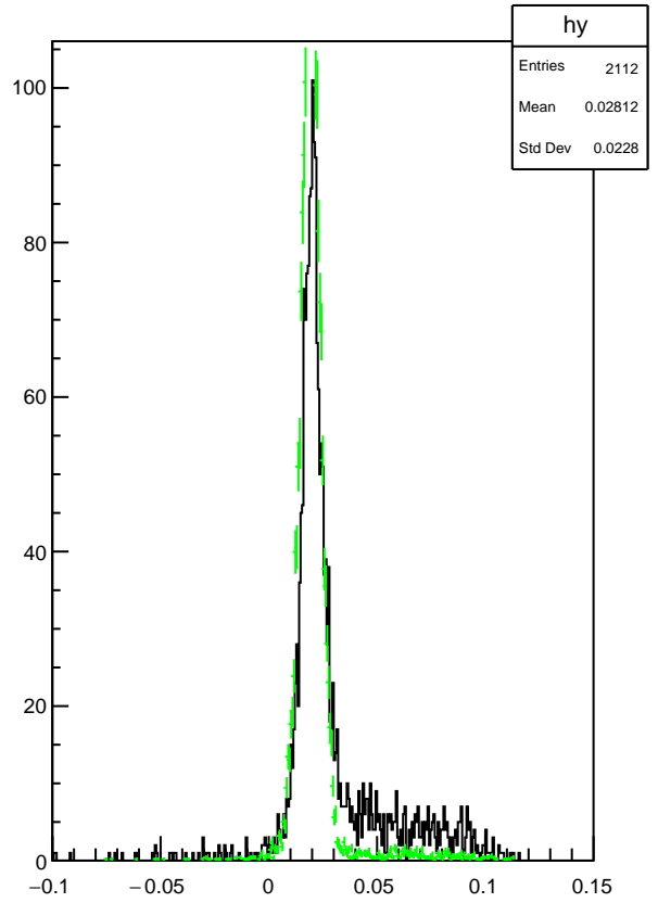
Plot 5 TwoPhotonAnalysis/Pi0_mmiss_acceptance 11
