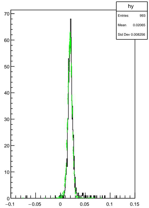
Plot 13 TwoPhotonAnalysis/Pi0_mmiss_final_vertex 19
