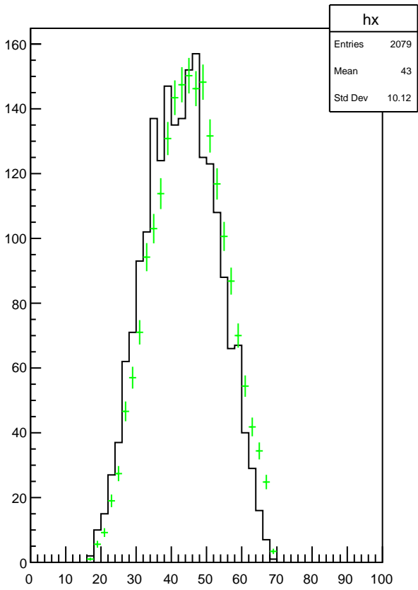
Plot 6 TwoPhotonAnalysis/Pi0_mmiss_isolation 12
