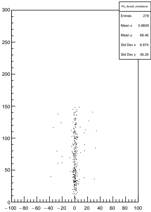
Plot 9 TwoPhotonAnalysis/Pic_lkrCELL_mindistvst 15
