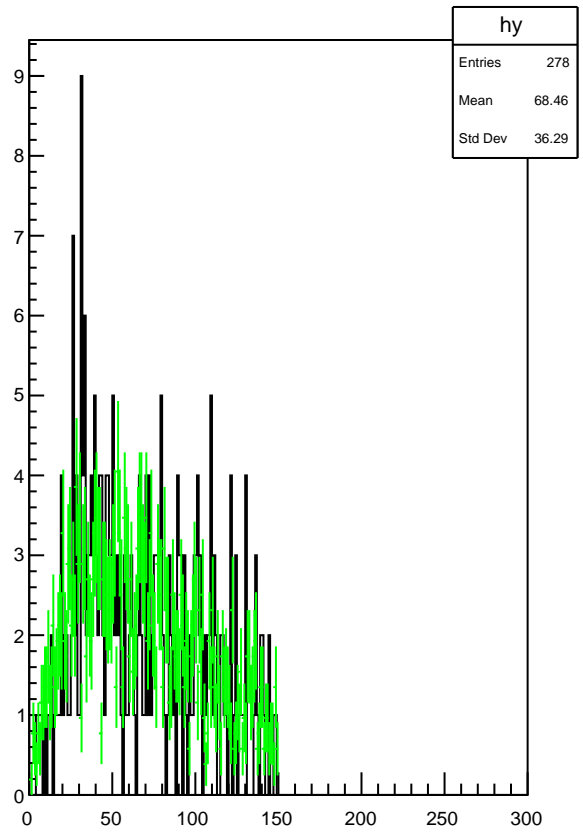
Plot 9 TwoPhotonAnalysis/Pic_lkrCELL_mindistvst 15
