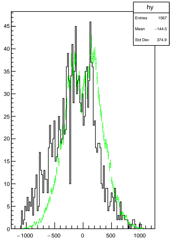
Plot 21 TwoPhotonAnalysis/EMClusterXY_high_pnn 33
