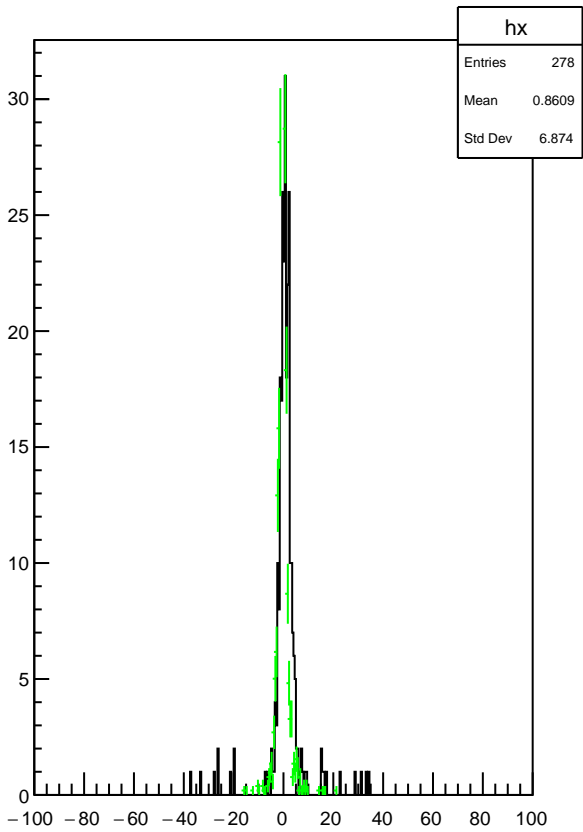
Plot 9 TwoPhotonAnalysis/Pic_lkrCELL_mindistvst 15
