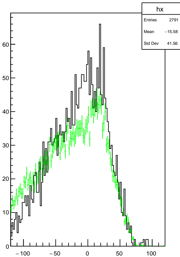
Plot 1 TwoPhotonAnalysis/Pic_posAtCHOD 5
