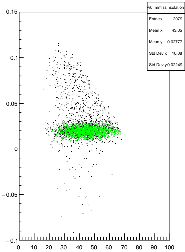
Plot 6 TwoPhotonAnalysis/Pi0_mmiss_isolation 12
