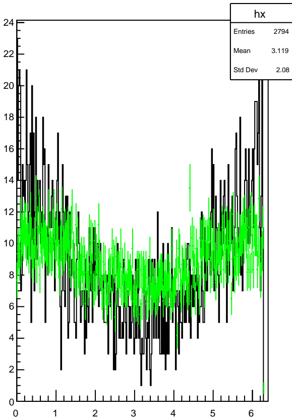
Plot 2 TwoPhotonAnalysis/Pi0_mmissVSPHi_pic 7
