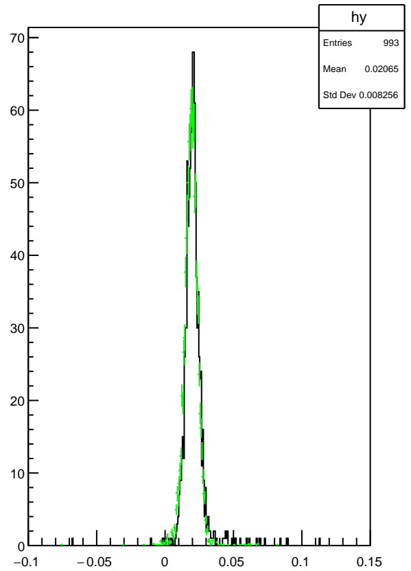
Plot 15 TwoPhotonAnalysis/Pi0_mmiss_final_trigg 21
