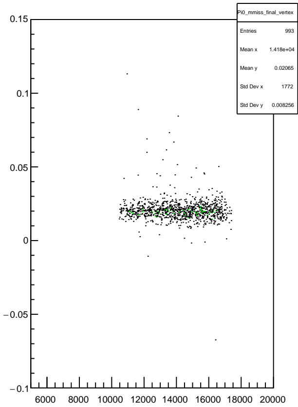
Plot 13 TwoPhotonAnalysis/Pi0_mmiss_final_vertex 19
