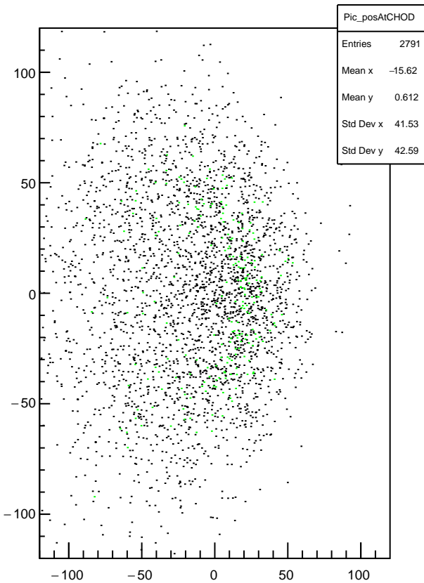
Plot 1 TwoPhotonAnalysis/Pic_posAtCHOD 5
