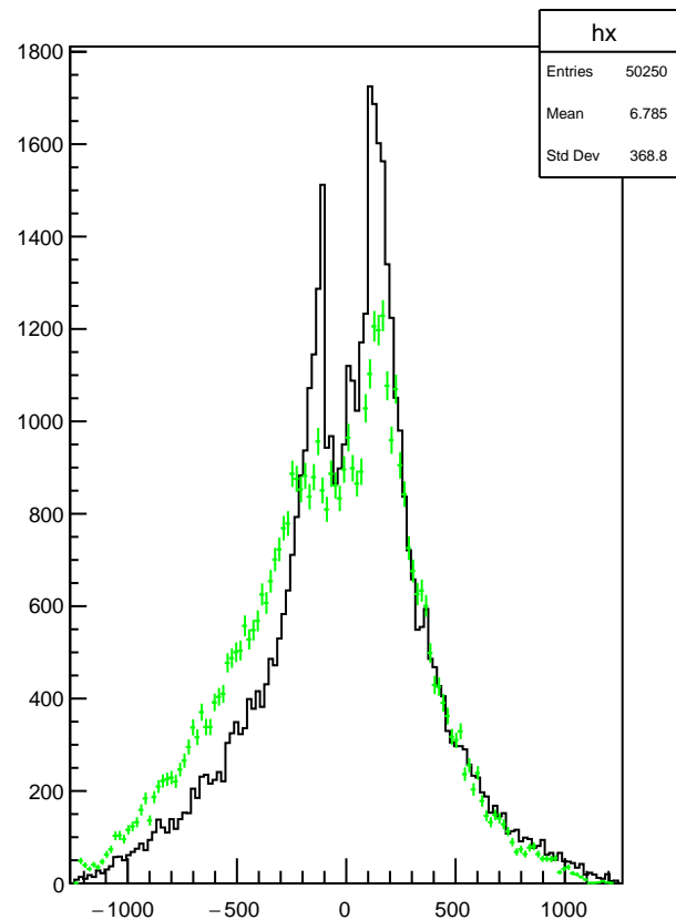
Plot 25 TwoPhotonAnalysis/OtherClusterXY 38
