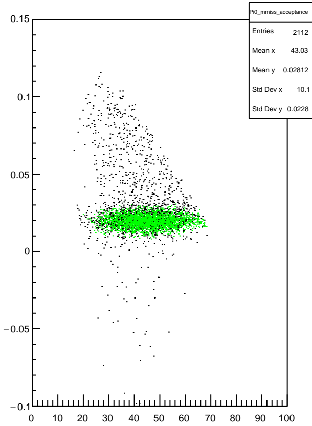
Plot 5 TwoPhotonAnalysis/Pi0_mmiss_acceptance 11
