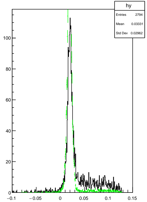
Plot 3 TwoPhotonAnalysis/Pi0_mmissVSPHi_pi0 8
