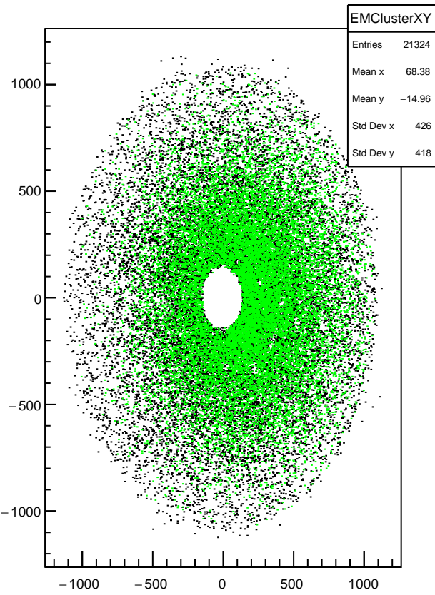
Plot 20 TwoPhotonAnalysis/EMClusterXY 32
