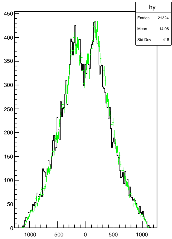
Plot 20 TwoPhotonAnalysis/EMClusterXY 32
