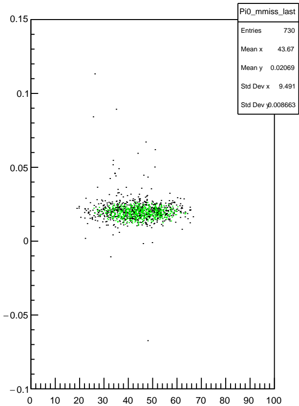
Plot 14 TwoPhotonAnalysis/Pi0_mmiss_last 20
