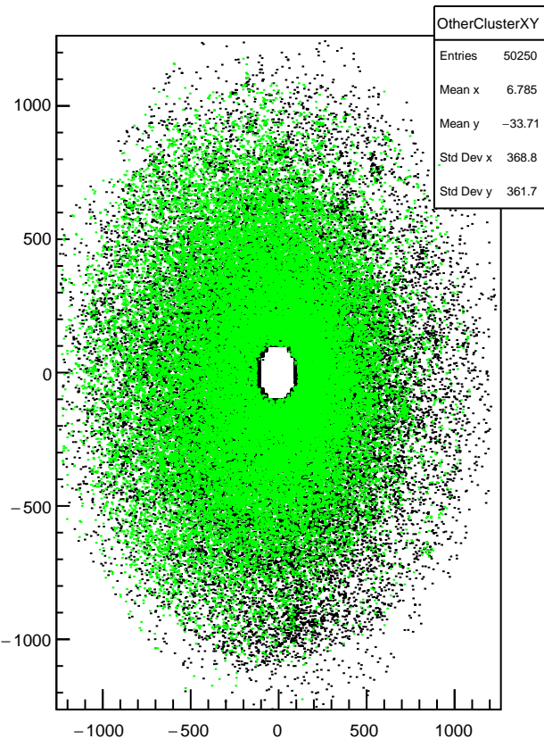
Plot 25 TwoPhotonAnalysis/OtherClusterXY 38
