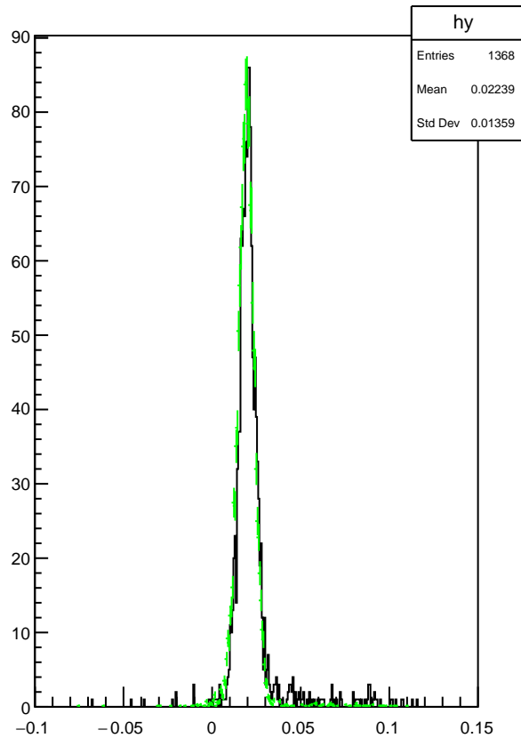
Plot 4 TwoPhotonAnalysis/Pi0_mmiss 9
