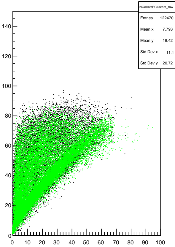
Plot 16 TwoPhotonAnalysis/NCellsvsEClusters_raw 25
