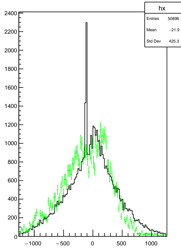
Plot 18 TwoPhotonAnalysis/MipClusterXY 29
