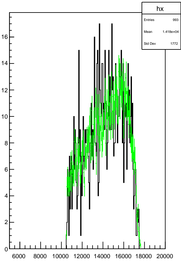
Plot 13 TwoPhotonAnalysis/Pi0_mmiss_final_vertex 19
