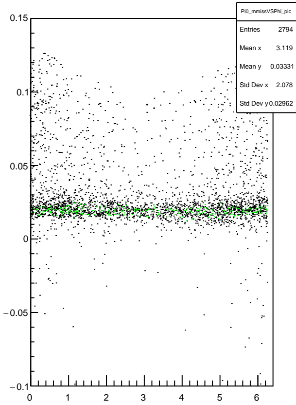
Plot 2 TwoPhotonAnalysis/Pi0_mmissVSPHi_pic 7
