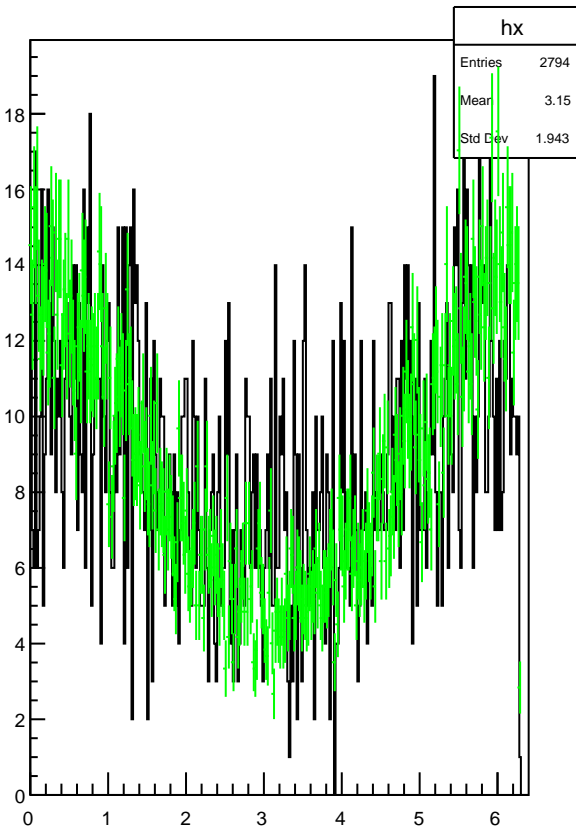
Plot 3 TwoPhotonAnalysis/Pi0_mmissVSPHi_pi0 8
