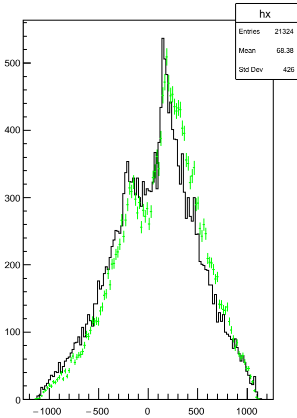
Plot 20 TwoPhotonAnalysis/EMClusterXY 32
