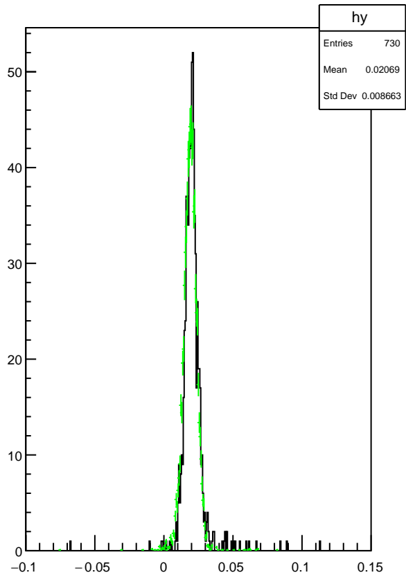
Plot 14 TwoPhotonAnalysis/Pi0_mmiss_last 20
