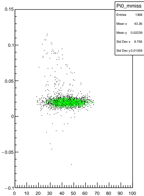
Plot 4 TwoPhotonAnalysis/Pi0_mmiss 9
