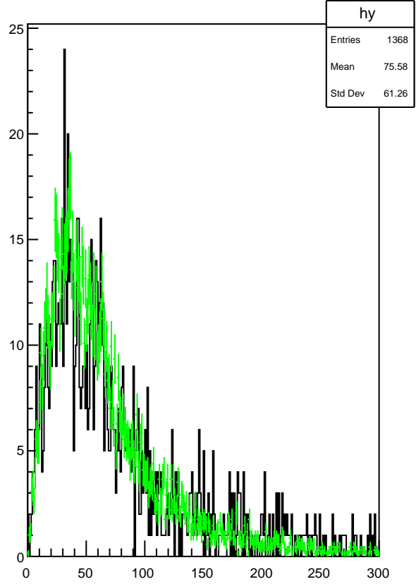
Plot 8 TwoPhotonAnalysis/Pic_lkrclus_mindistvst 14
