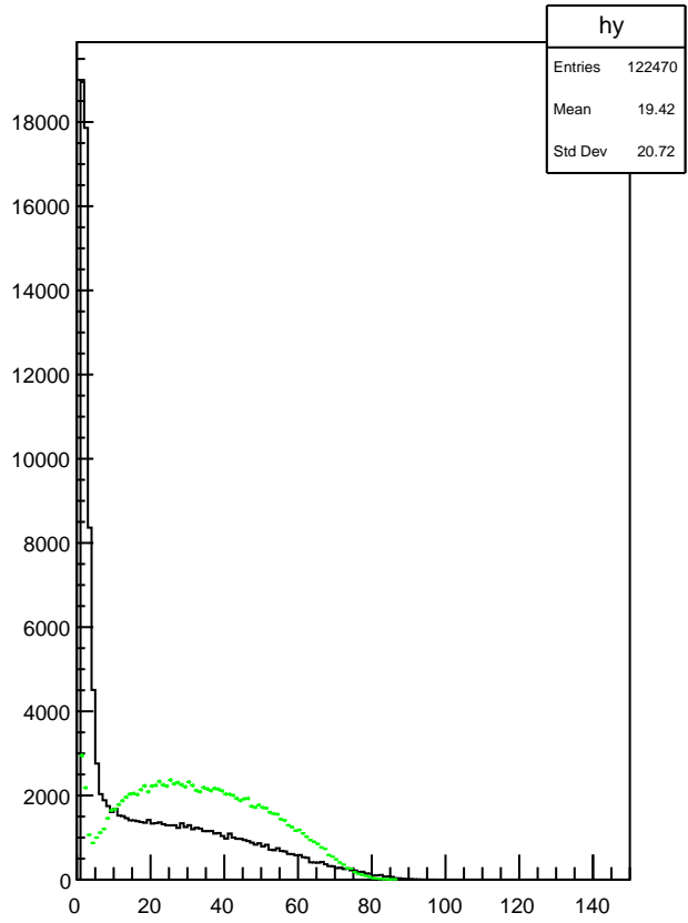
Plot 16 TwoPhotonAnalysis/NCellsvsEClusters_raw 25
