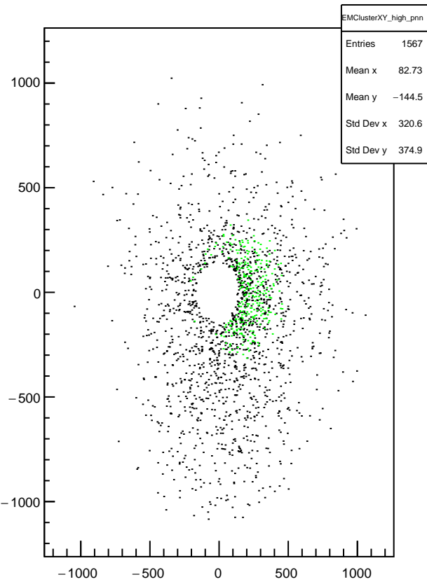
Plot 21 TwoPhotonAnalysis/EMClusterXY_high_pnn 33
