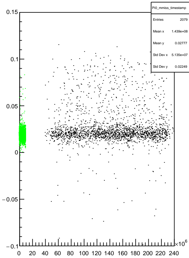
Plot 7 TwoPhotonAnalysis/Pi0_mmiss_timestamp 13
