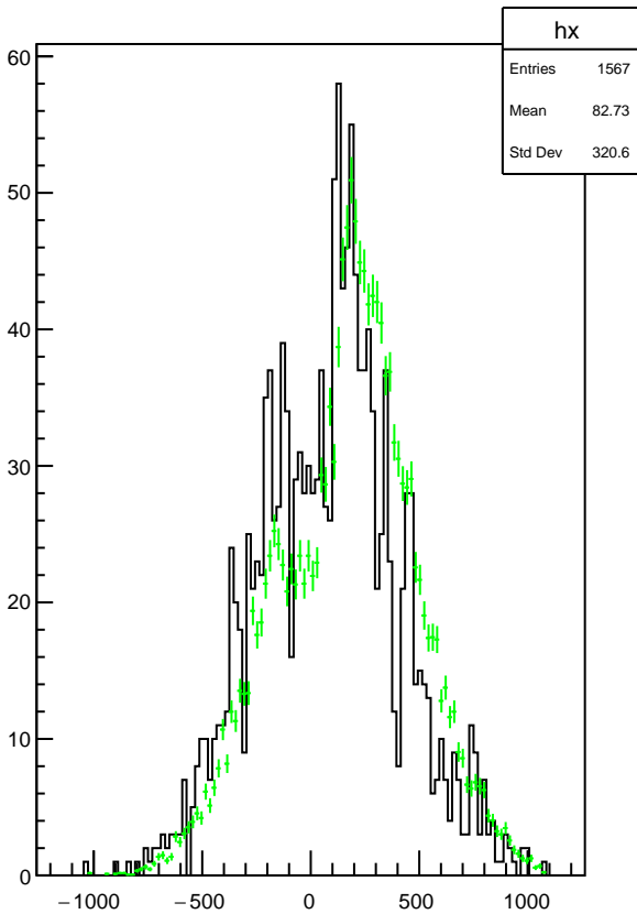
Plot 21 TwoPhotonAnalysis/EMClusterXY_high_pnn 33
