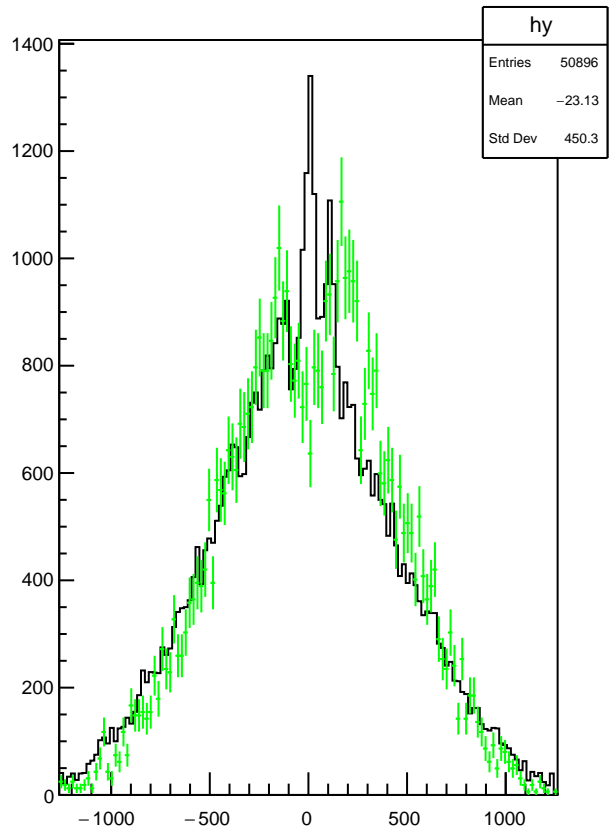
Plot 18 TwoPhotonAnalysis/MipClusterXY 29
