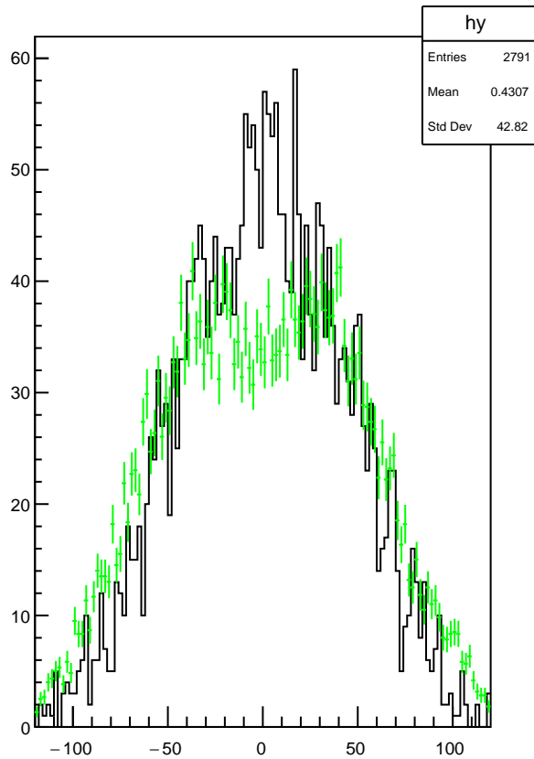
Plot 1 TwoPhotonAnalysis/Pic_posAtCHOD 5
