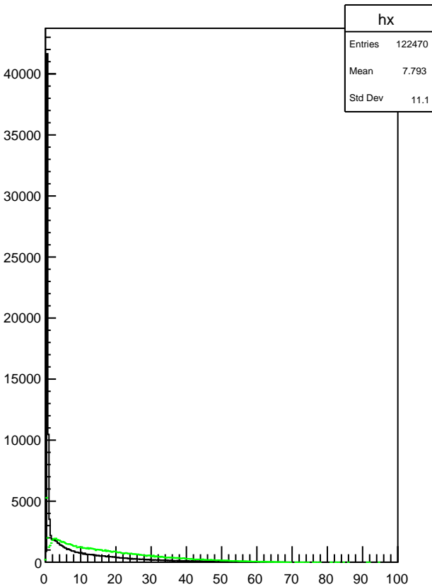
Plot 16 TwoPhotonAnalysis/NCellsvsEClusters_raw 25
