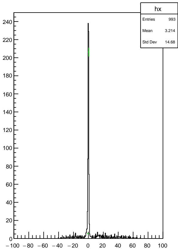
Plot 15 TwoPhotonAnalysis/Pi0_mmiss_final_trigg 21
