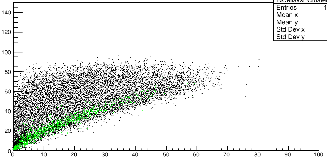
Plot 10 TwoPhotonAnalysis/NCellsvsEClusters_raw
