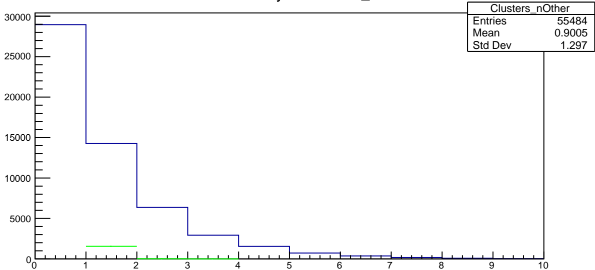
Plot 26 TwoPhotonAnalysis/Clusters_nOther 41
