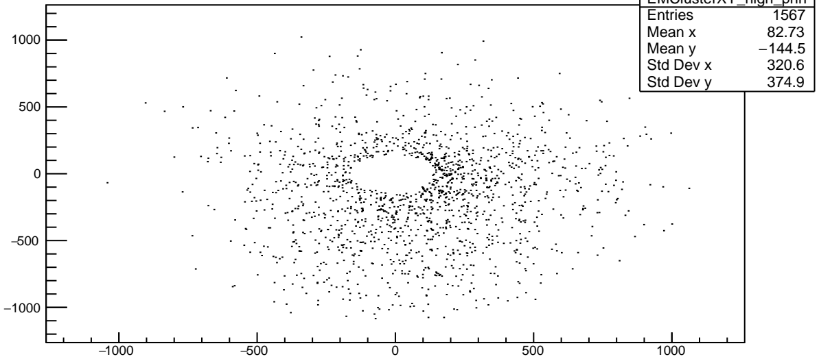
Plot 18 TwoPhotonAnalysis/EMClusterXY_high_pnn
