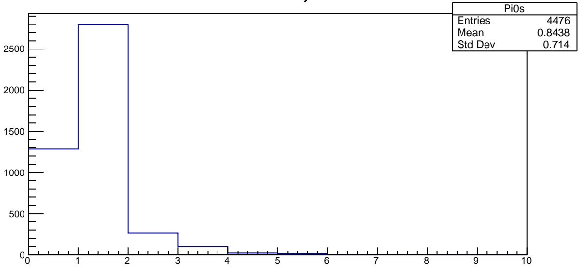
Plot 2 TwoPhotonAnalysis/Pi0s 3
