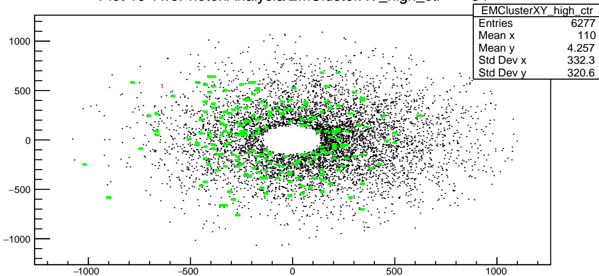
Plot 19 TwoPhotonAnalysis/EMClusterXY_high_ctr
