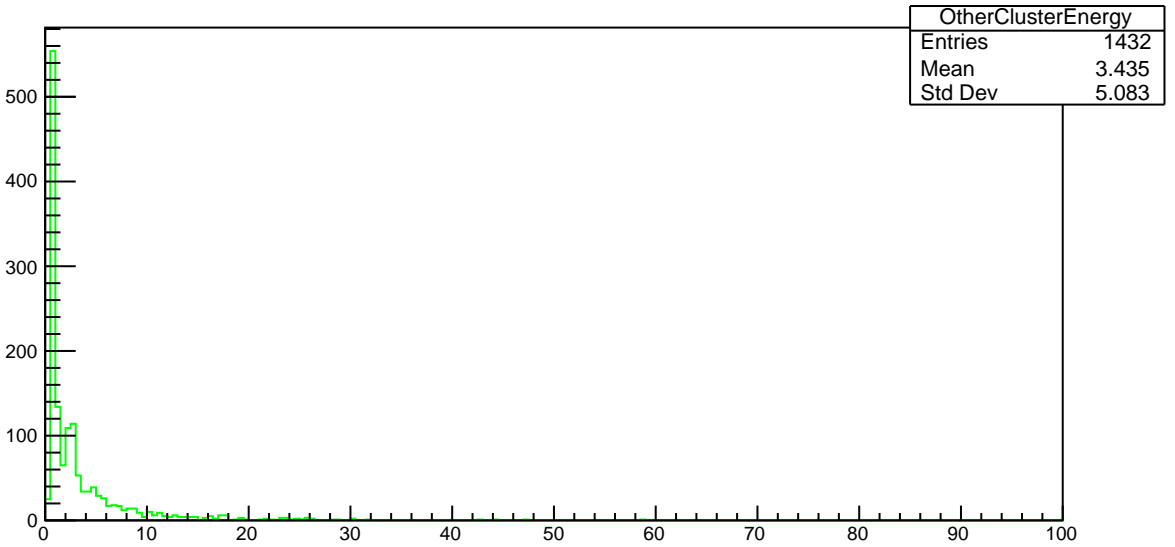
Plot 22 TwoPhotonAnalysis/OtherClusterEnergy 37
