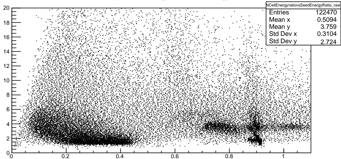
Plot 11 TwoPhotonAnalysis/NCellEnergyrativsSeedEnergyRatio_raw
