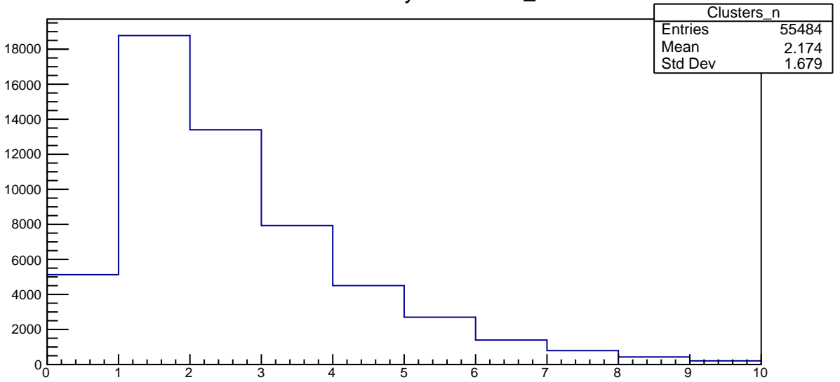
Plot 8 TwoPhotonAnalysis/Clusters_n 23
