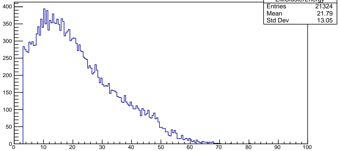
Plot 16 TwoPhotonAnalysis/EMClusterEnergy 31
