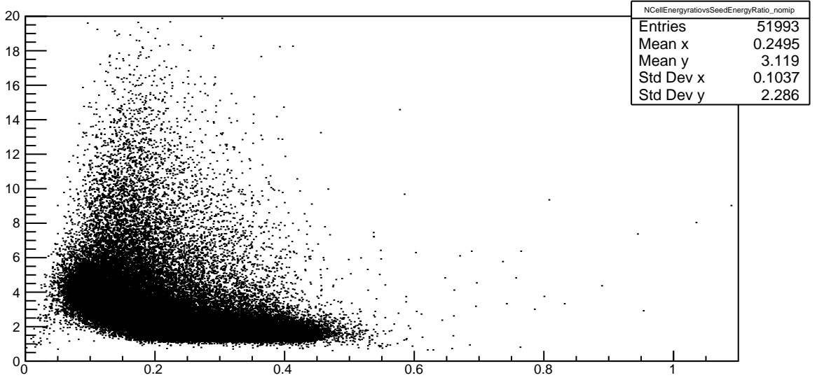
Plot 15 TwoPhotonAnalysis/NCellEnergyrativovsSeedEnergyRatio_nomip 30
