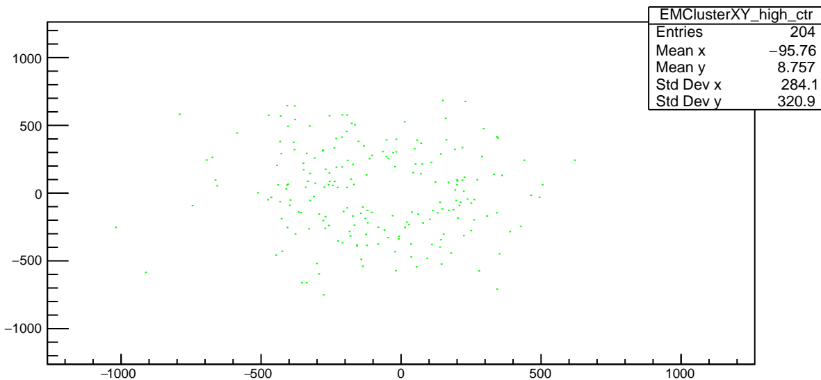
Plot 19 TwoPhotonAnalysis/EMClusterXY_high_ctr
