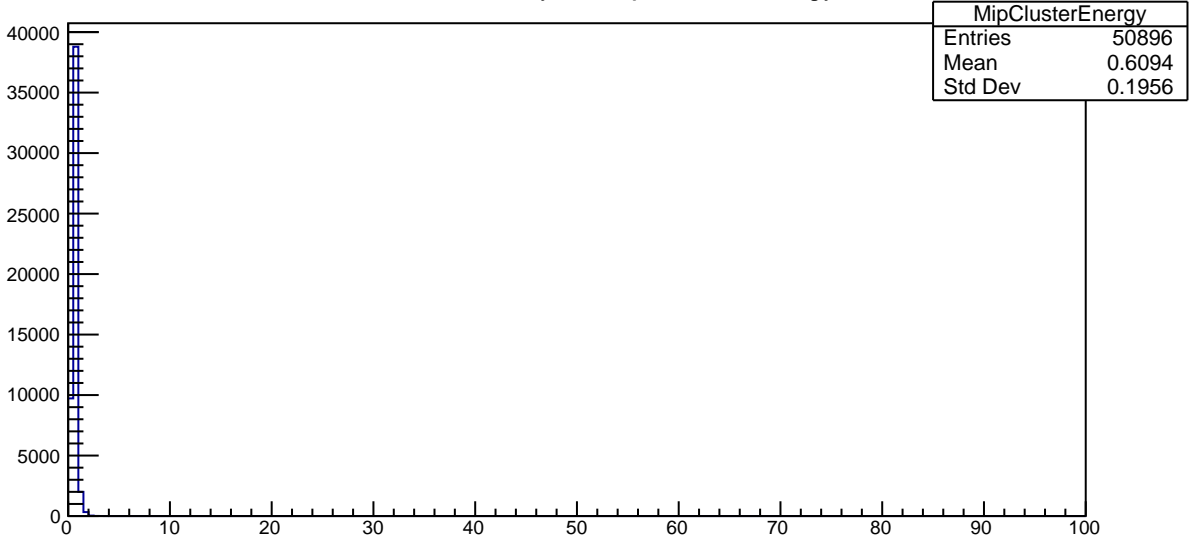
Plot 12 TwoPhotonAnalysis/MipClusterEnergy 27
