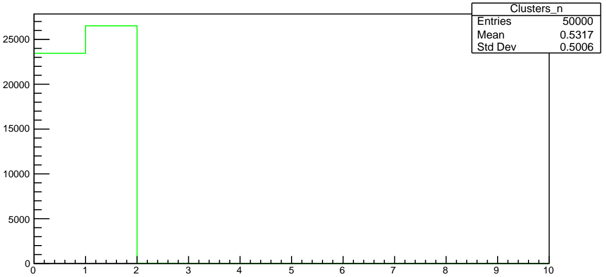
Plot 8 TwoPhotonAnalysis/Clusters_n 23
