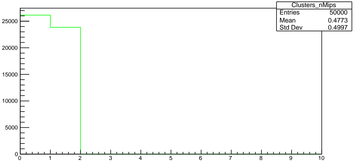
Plot 24 TwoPhotonAnalysis/Clusters_nMips 39
