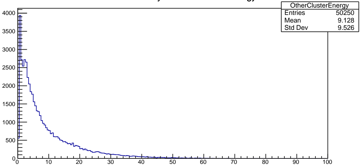
Plot 22 TwoPhotonAnalysis/OtherClusterEnergy 37
