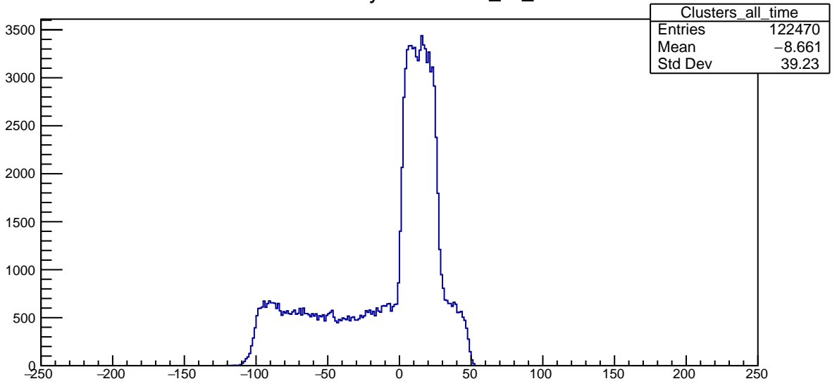
Plot 9 TwoPhotonAnalysis/Clusters_all_time 24
