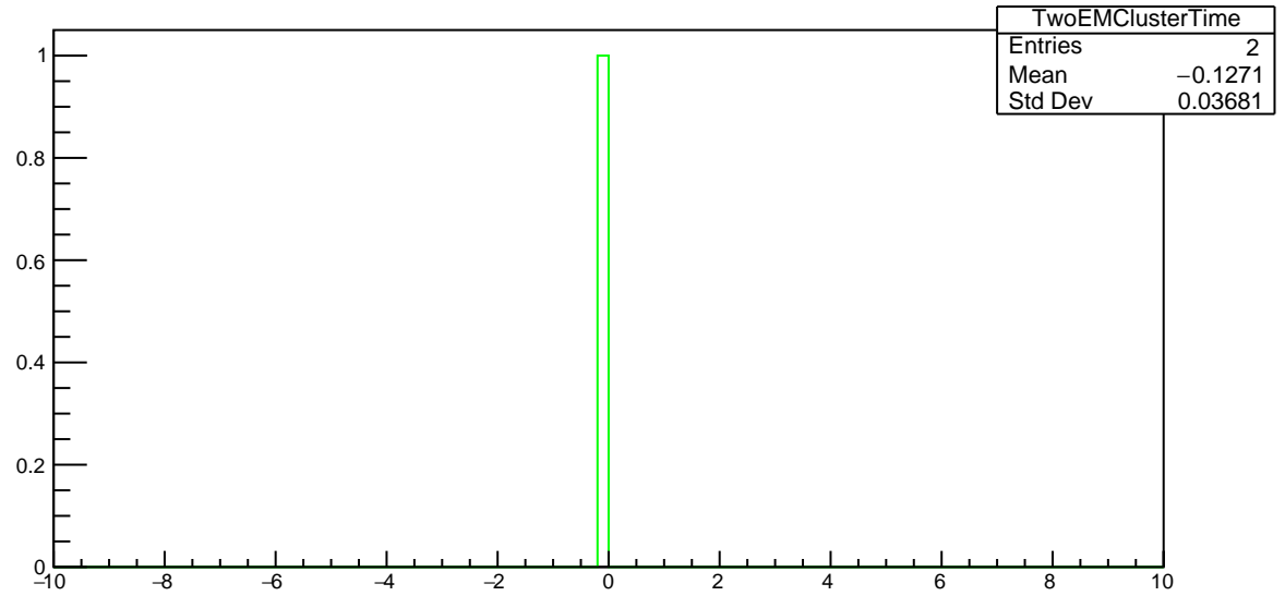
Plot 27 TwoPhotonAnalysis/TwoEMClusterTime
