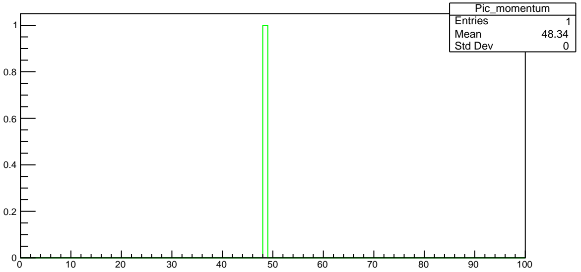
Plot 3 TwoPhotonAnalysis/Pic_momentum 4
