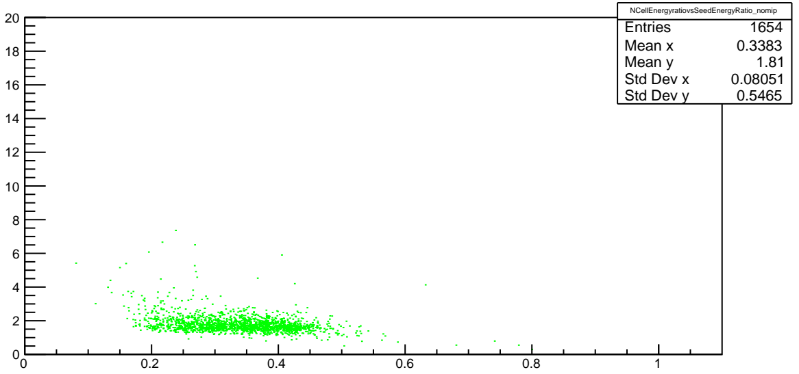
Plot 15 TwoPhotonAnalysis/NCellEnergyrativovsSeedEnergyRatio_nomip 30
