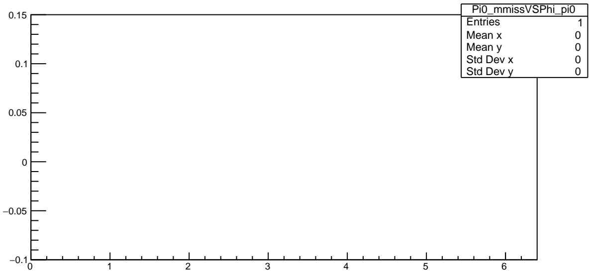
Plot 7 TwoPhotonAnalysis/Pi0_mmissVSPhi_pi0
