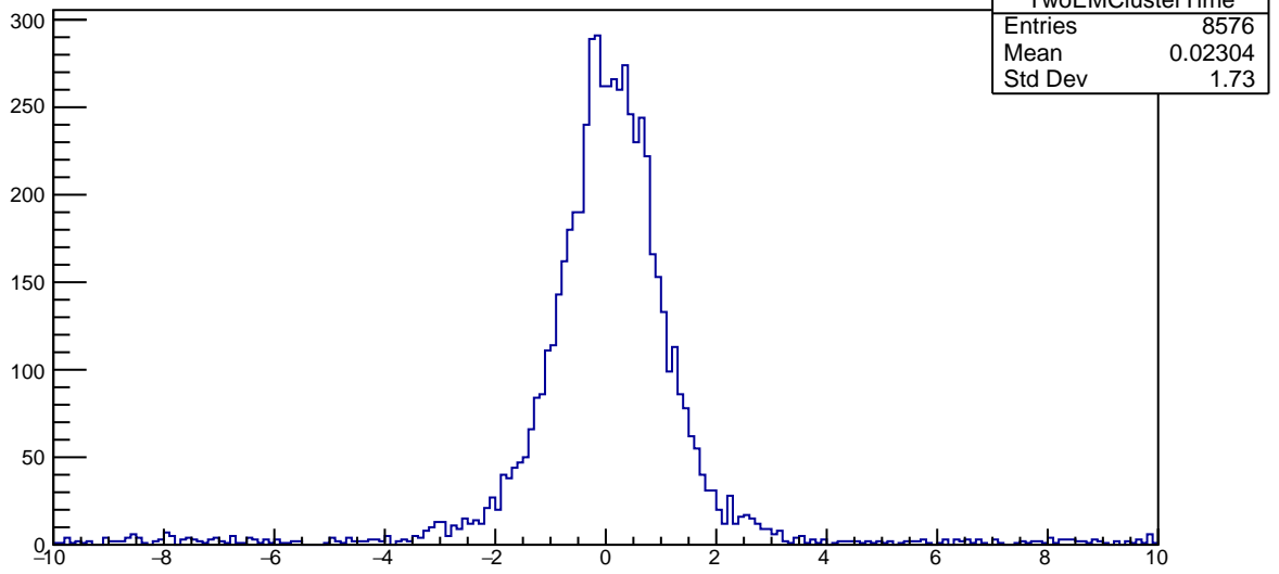
Plot 27 TwoPhotonAnalysis/TwoEMClusterTime
