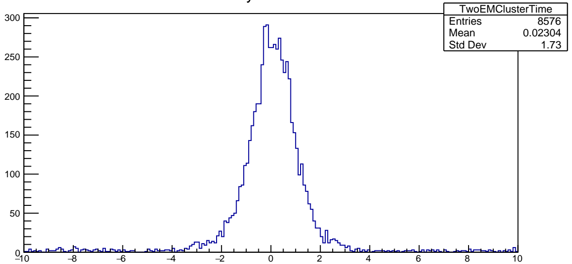
Plot 27 TwoPhotonAnalysis/TwoEMClusterTime
