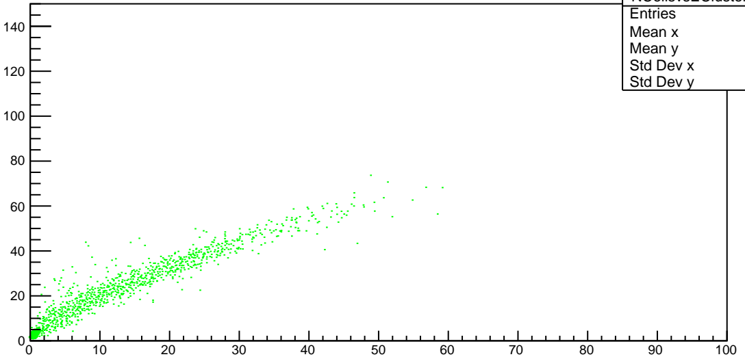
Plot 10 TwoPhotonAnalysis/NCellsvsEClusters_raw
