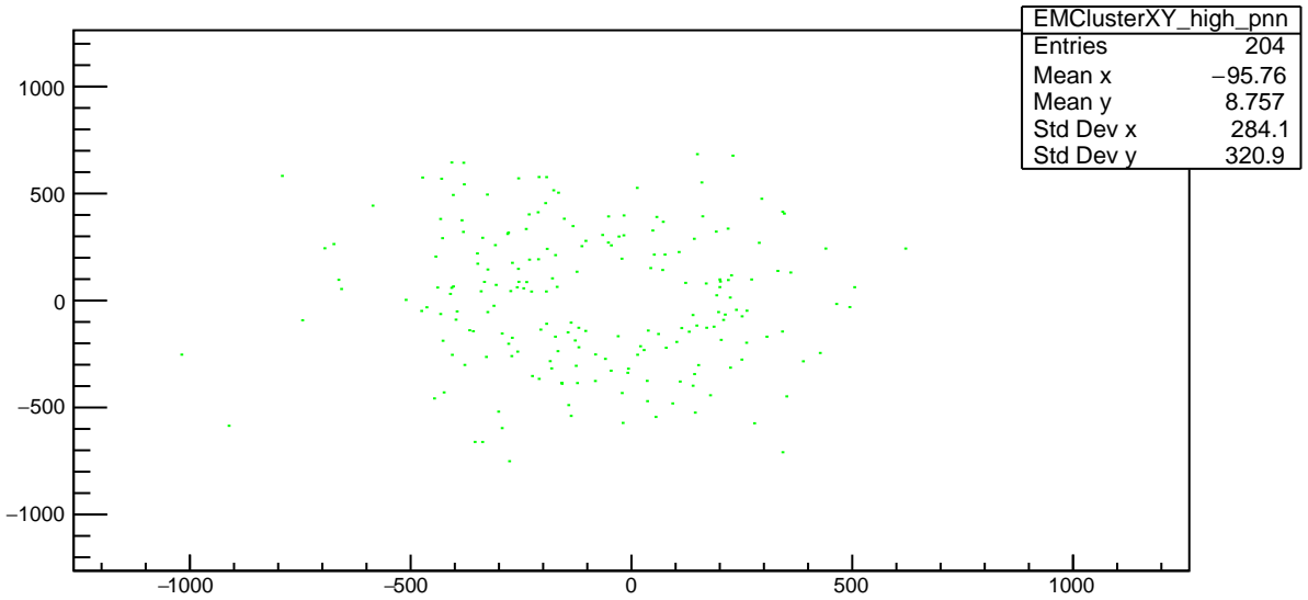
Plot 18 TwoPhotonAnalysis/EMClusterXY_high_pnn
