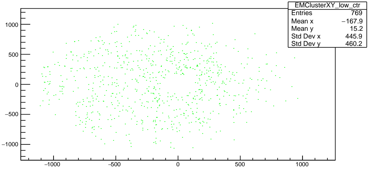
Plot 21 TwoPhotonAnalysis/EMClusterXY_low_ctr
