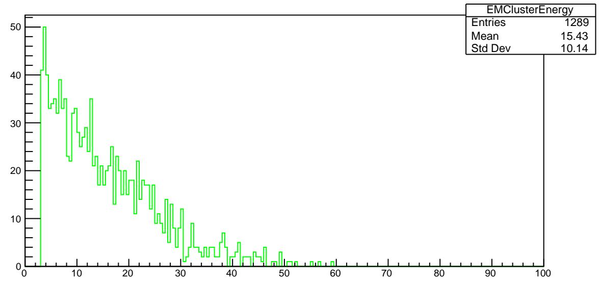
Plot 16 TwoPhotonAnalysis/EMClusterEnergy 31
