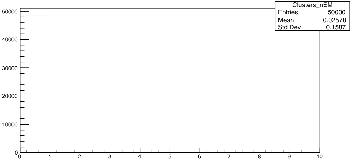
Plot 25 TwoPhotonAnalysis/Clusters_nEM 40
