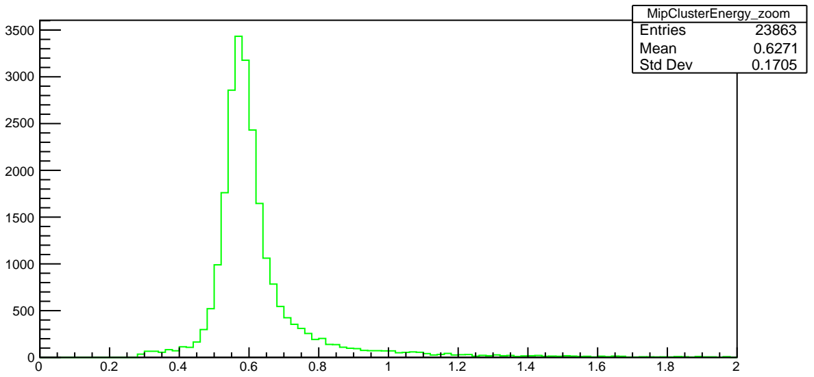
Plot 13 TwoPhotonAnalysis/MipClusterEnergy_zoom
