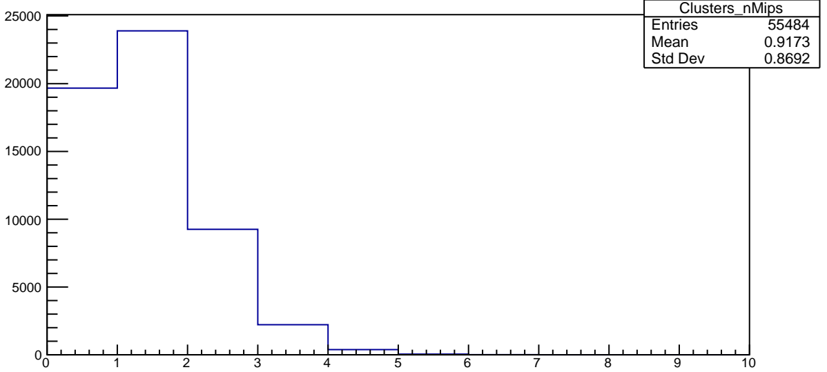
Plot 24 TwoPhotonAnalysis/Clusters_nMips 39
