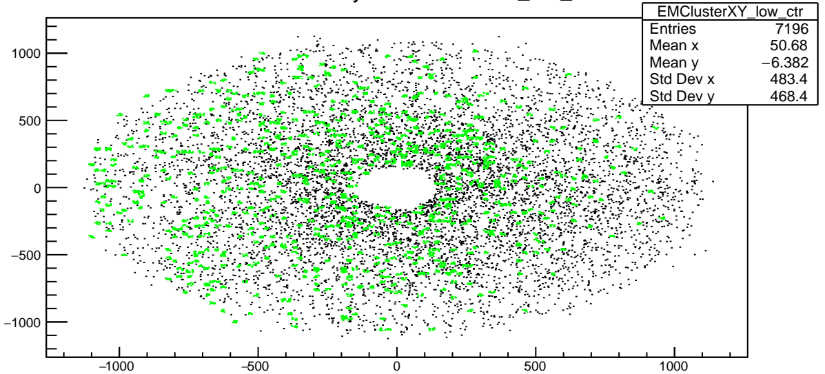
Plot 21 TwoPhotonAnalysis/EMClusterXY_low_ctr
