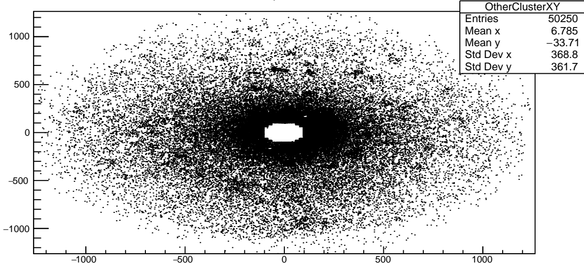
Plot 23 TwoPhotonAnalysis/OtherClusterXY 38
