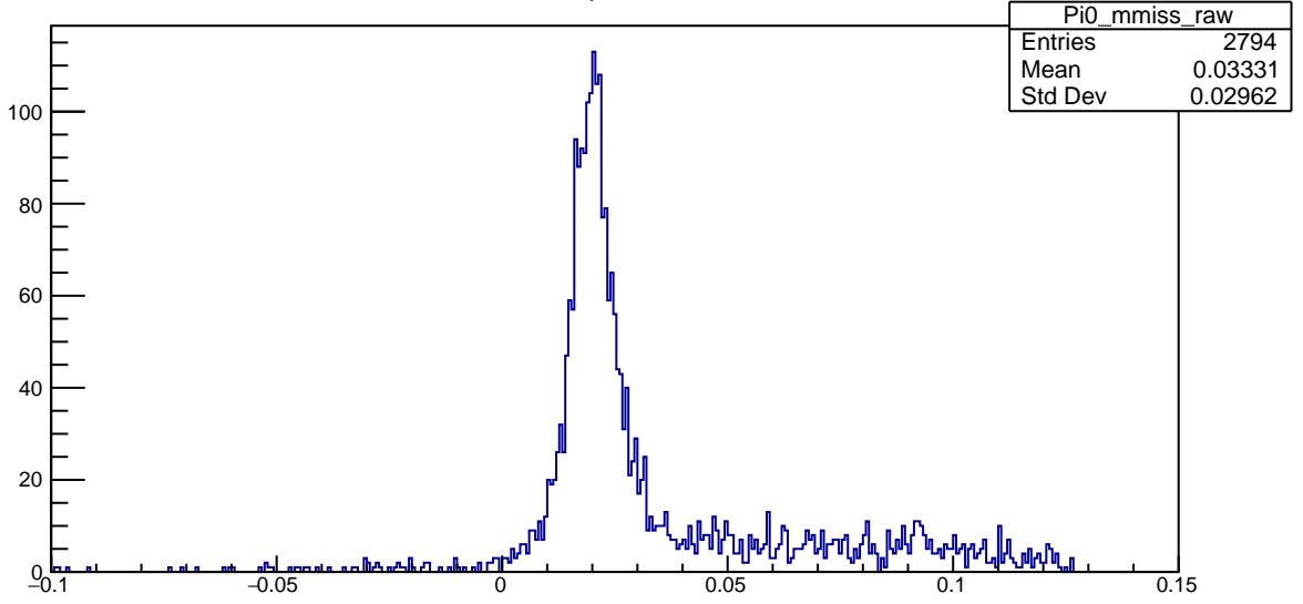
Plot 5 TwoPhotonAnalysis/Pi0_mmiss_raw 6
