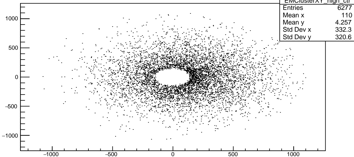
Plot 19 TwoPhotonAnalysis/EMClusterXY_high_ctr
