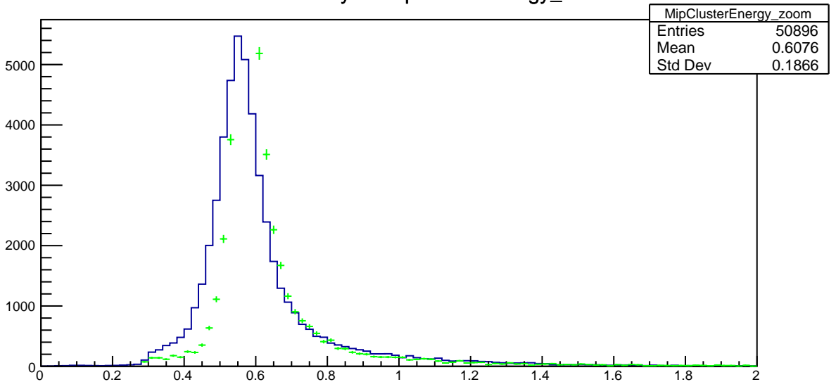
Plot 13 TwoPhotonAnalysis/MipClusterEnergy_zoom
