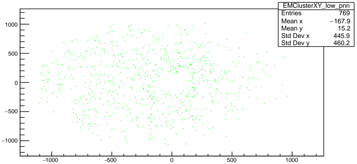
Plot 20 TwoPhotonAnalysis/EMClusterXY_low_pnn
