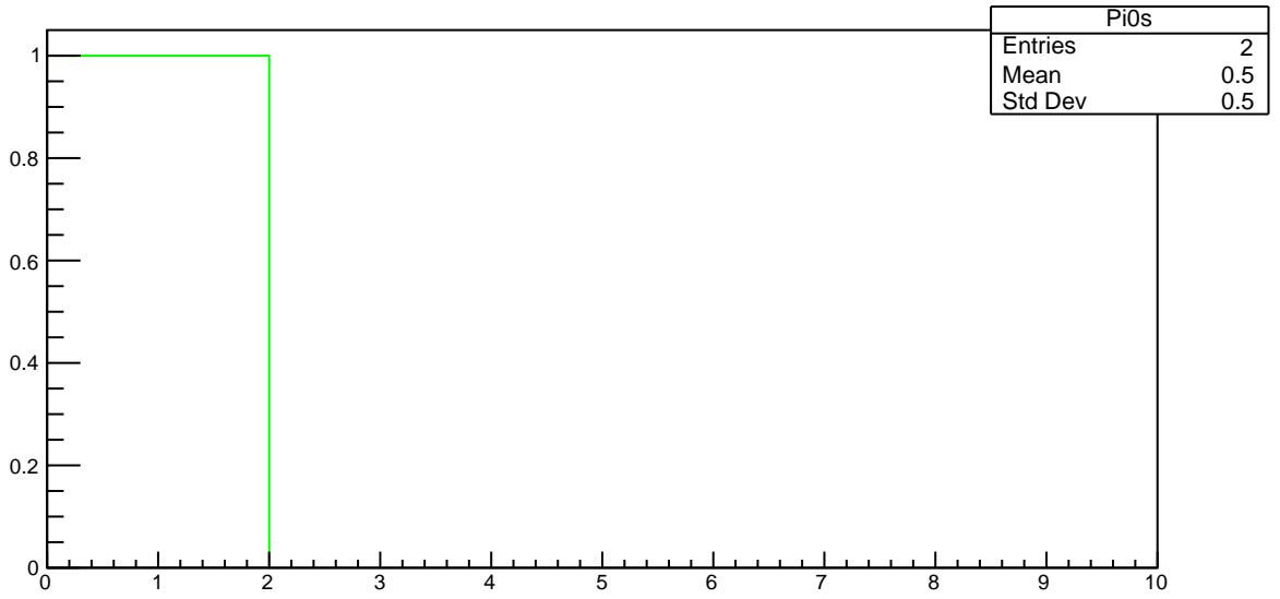
Plot 2 TwoPhotonAnalysis/Pi0s 3
