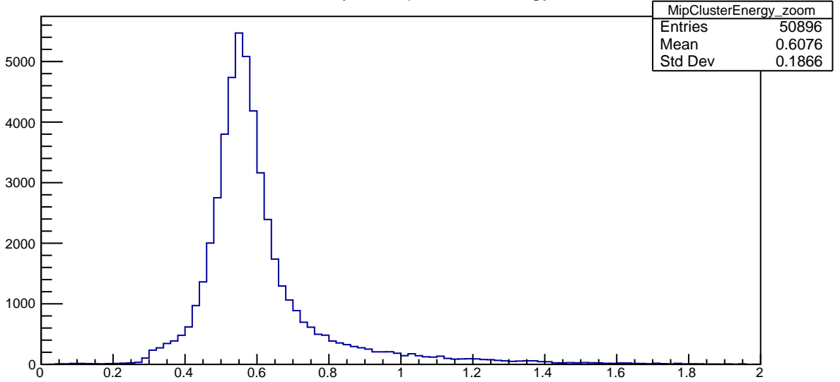
Plot 13 TwoPhotonAnalysis/MipClusterEnergy_zoom
