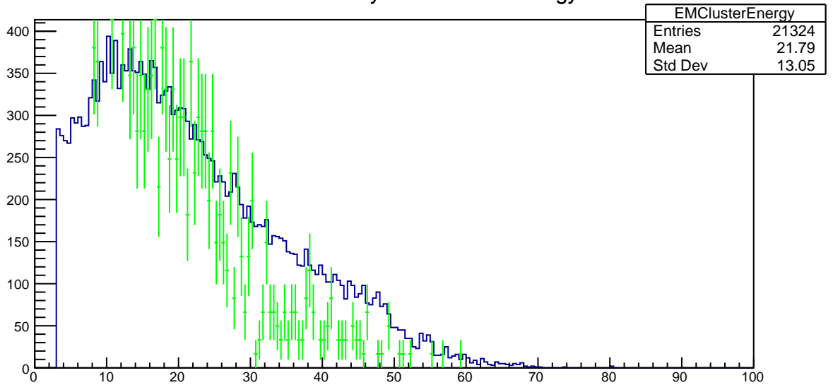
Plot 16 TwoPhotonAnalysis/EMClusterEnergy 31
