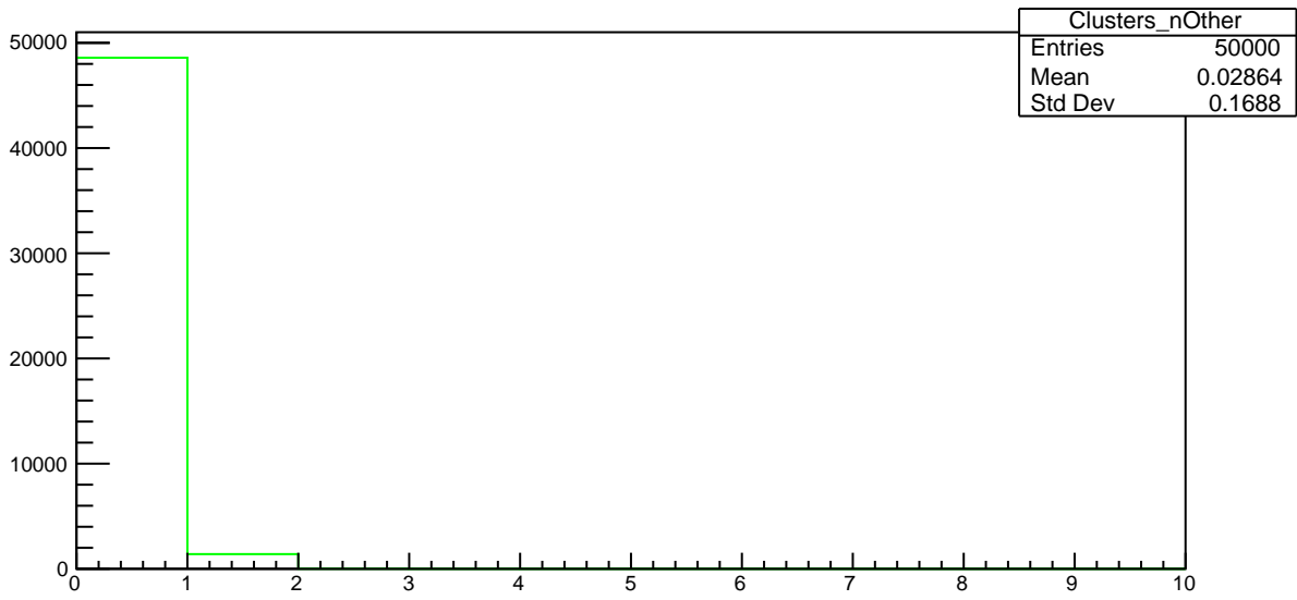
Plot 26 TwoPhotonAnalysis/Clusters_nOther 41
