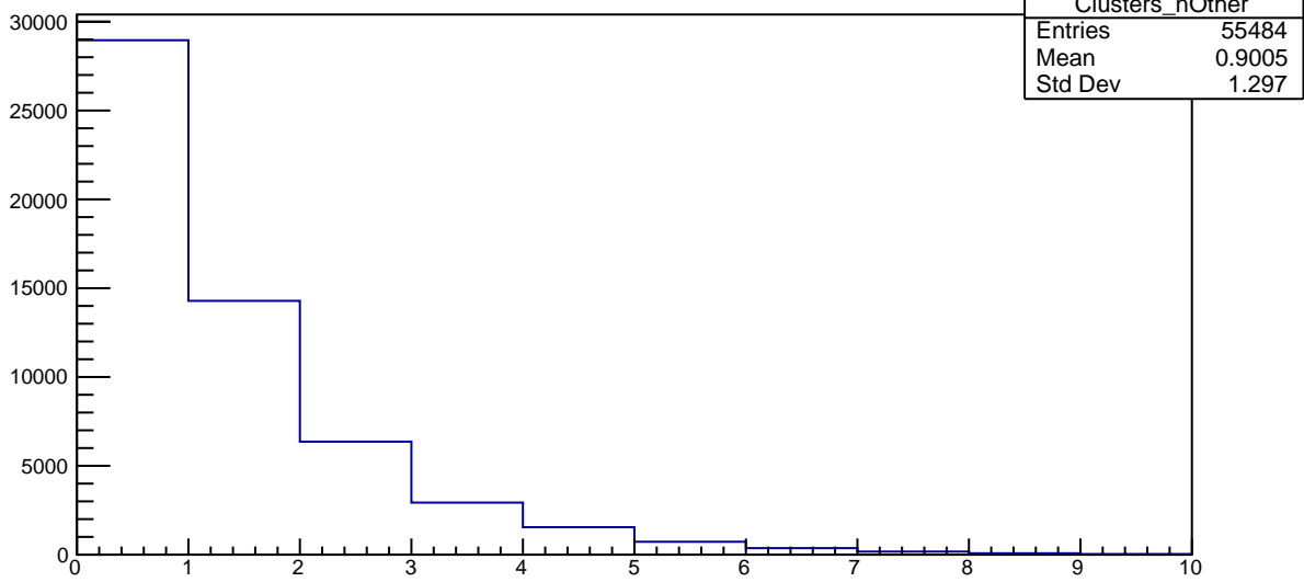
Plot 26 TwoPhotonAnalysis/Clusters_nOther 41
