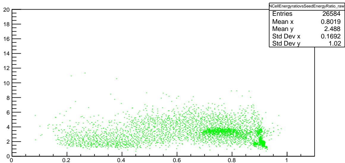
Plot 11 TwoPhotonAnalysis/NCellEnergyrativsSeedEnergyRatio_raw
