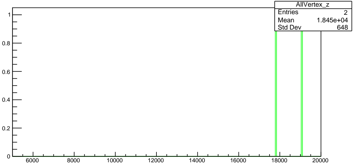
Plot 1 TwoPhotonAnalysis/AllVertex_z 2
