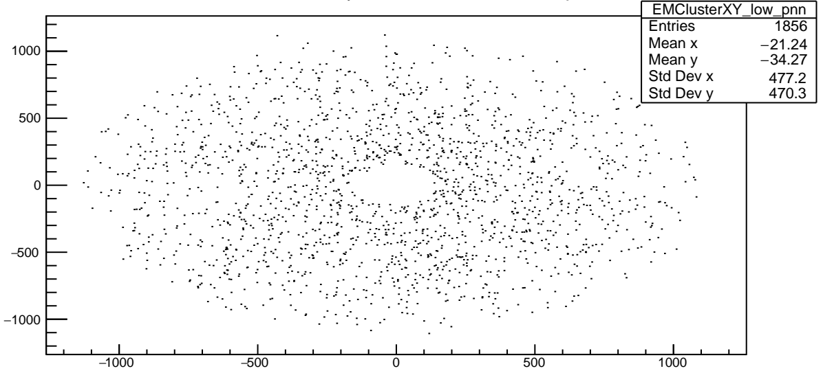
Plot 20 TwoPhotonAnalysis/EMClusterXY_low_pnn
