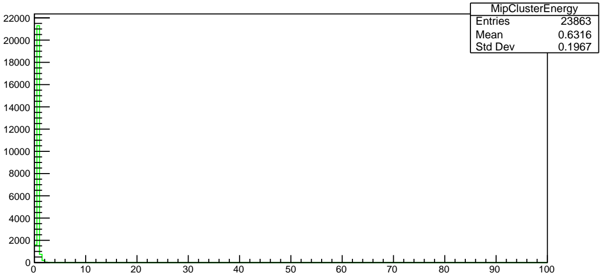
Plot 12 TwoPhotonAnalysis/MipClusterEnergy 27
