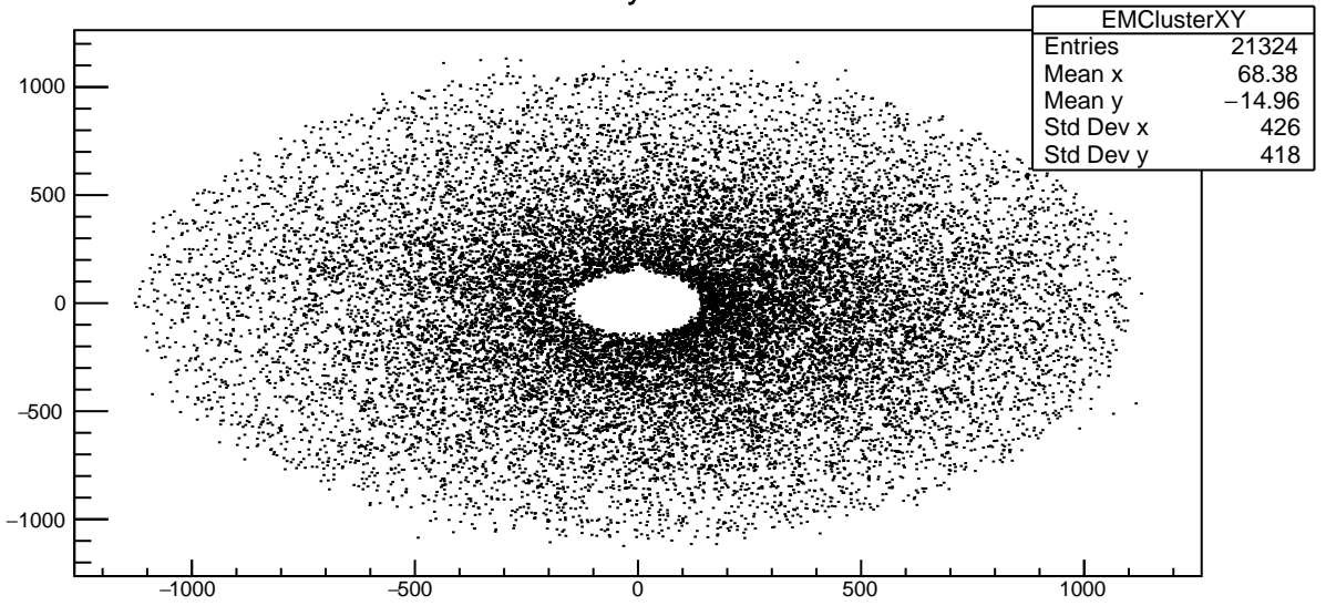
Plot 17 TwoPhotonAnalysis/EMClusterXY 32
