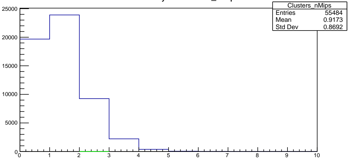
Plot 24 TwoPhotonAnalysis/Clusters_nMips 39
