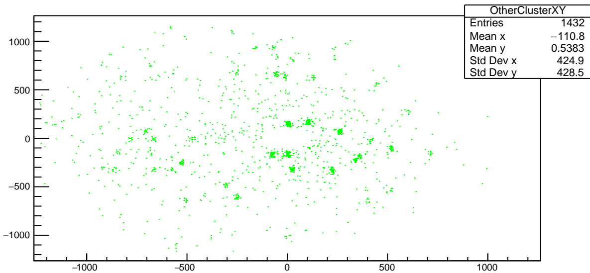
Plot 23 TwoPhotonAnalysis/OtherClusterXY 38
