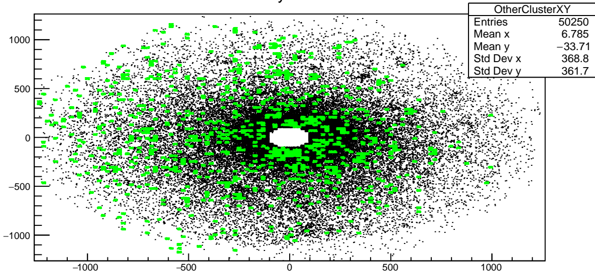
Plot 23 TwoPhotonAnalysis/OtherClusterXY 38
