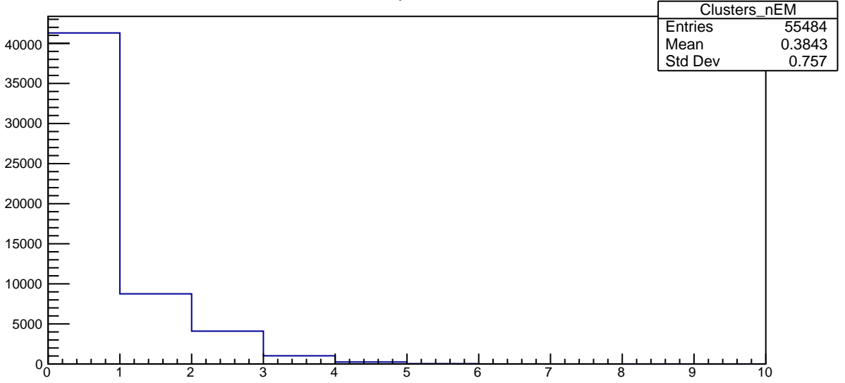
Plot 25 TwoPhotonAnalysis/Clusters_nEM 40
