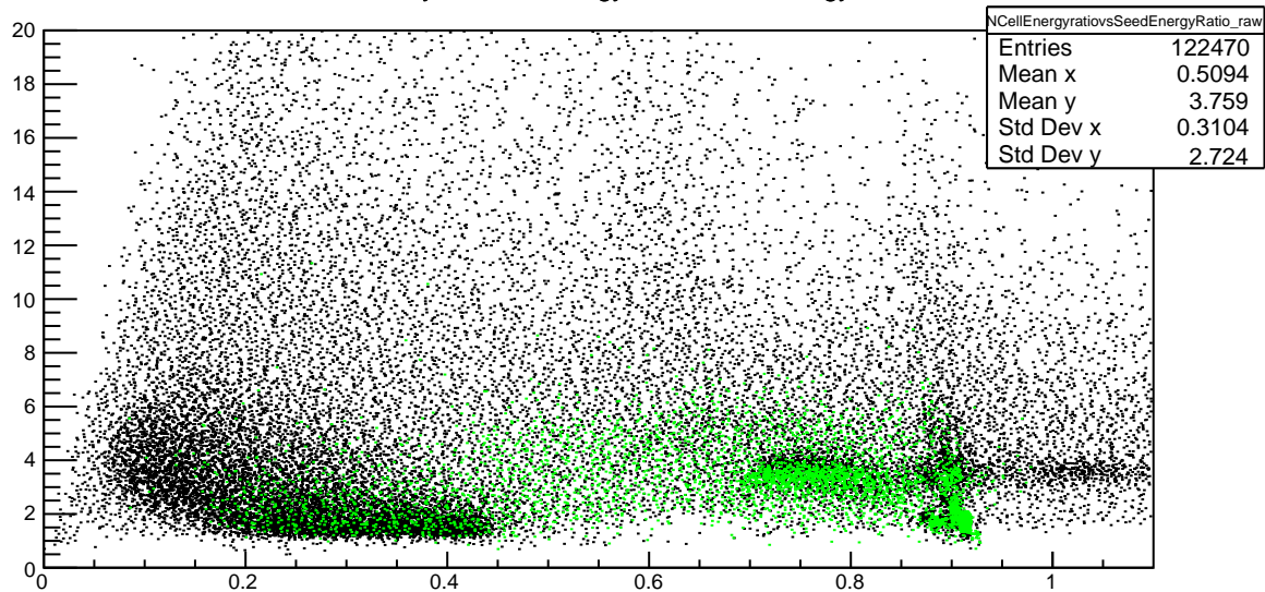
Plot 11 TwoPhotonAnalysis/NCellEnergyrativsSeedEnergyRatio_raw
