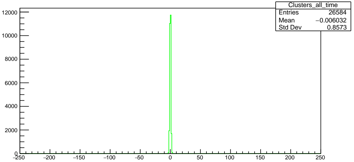
Plot 9 TwoPhotonAnalysis/Clusters_all_time 24
