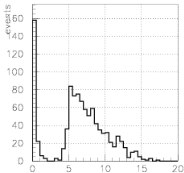
pt electron
