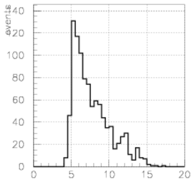
pt gamma
