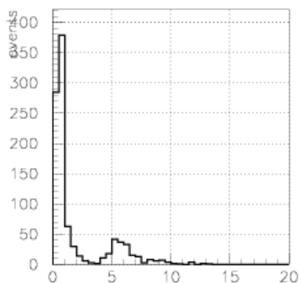
pt hadrons
