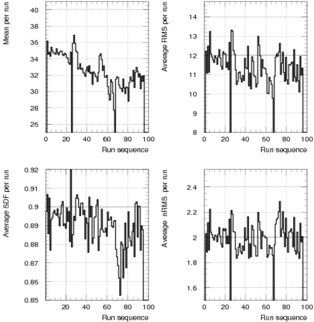
Mean, RMS, SDF, nRMS of Spill vs run sequence 14400 -14523
