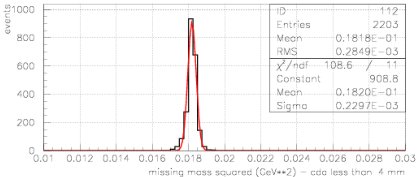
Least squares fit, K \pi 2 decay, 4C fit MC
