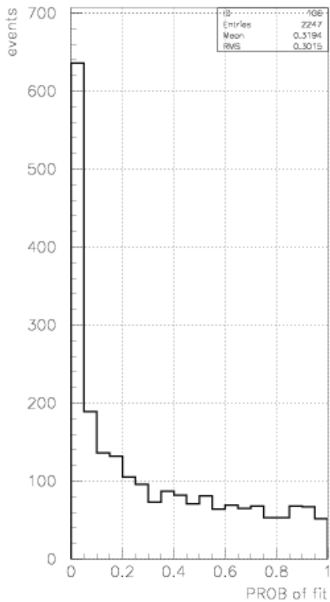
Least squares fit, K \pi 2 decay, 4C fit MC
