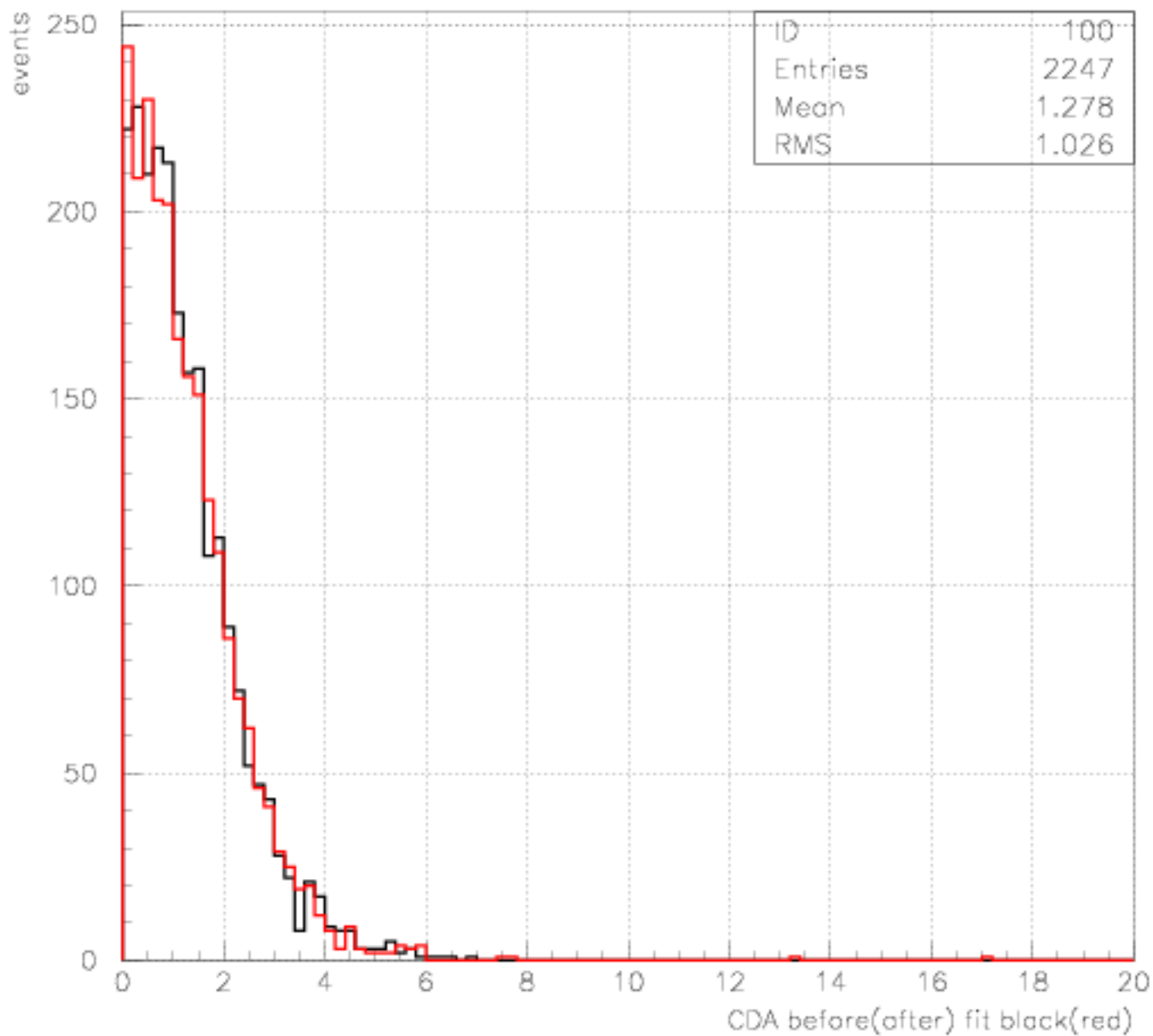
Least squares fit, K\pi^2 decay, 4C fit MC
