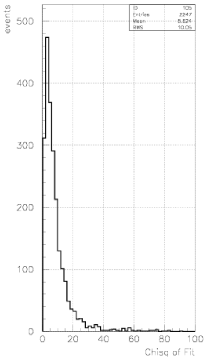
Least squares fit, K \pi 2 decay, 4C fit MC
