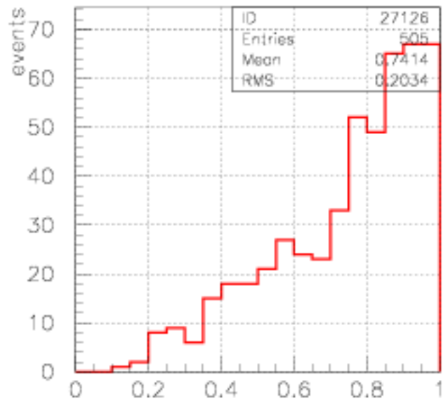
x-gamma no electron
