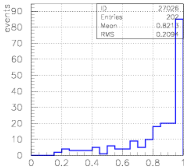
xgamma electron
