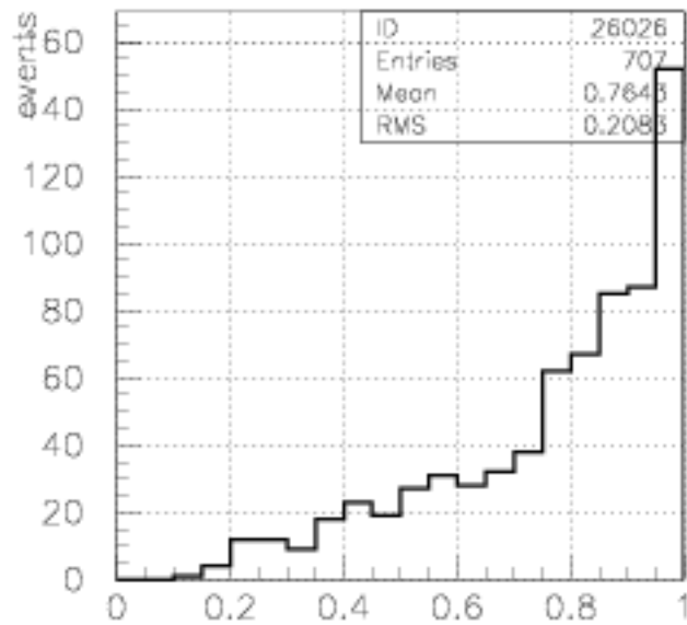
x-gamma all events
