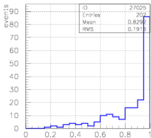
Zp electron
