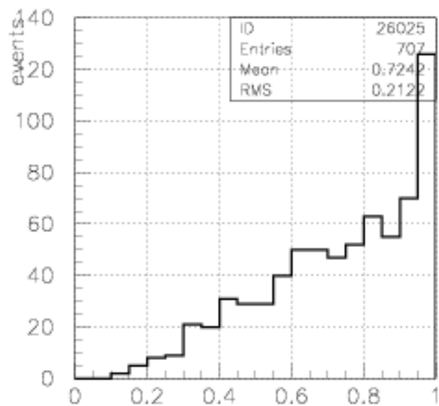
Zp all events
