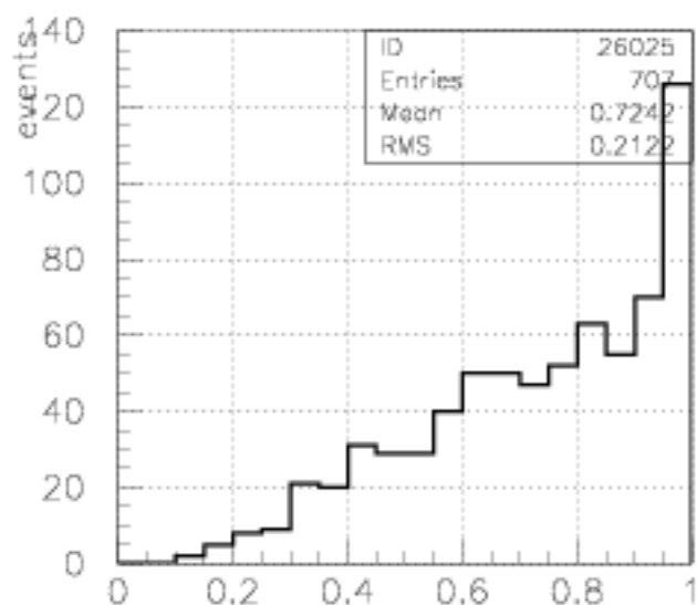
Zp all events
