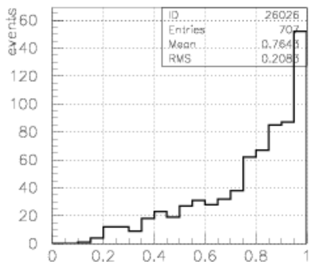
x-gamma all events
