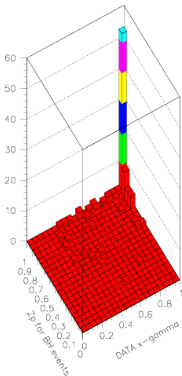
(3) LHS BH events, RHS after BH rejection
