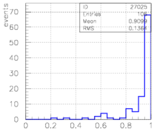
Zp rejected
