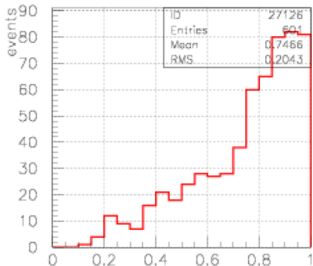
x-gamma selected
