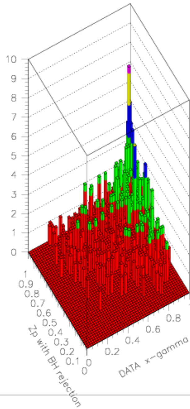
(2) LHS BH events, RHS after BH rejection
