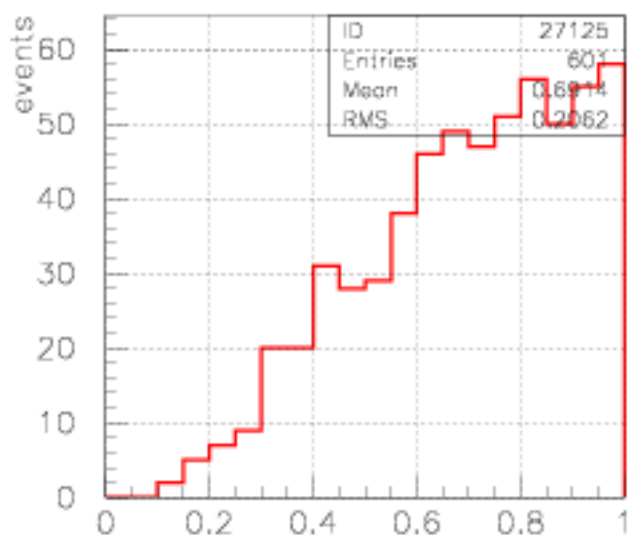
Zp selected
