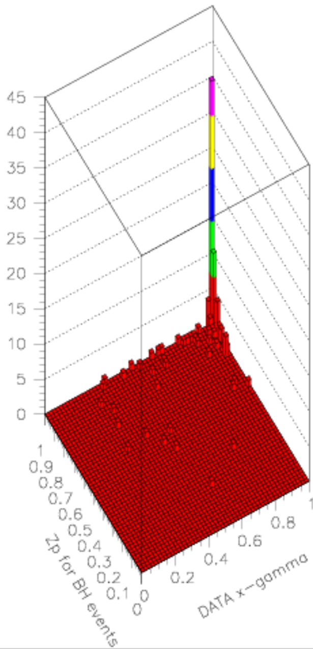
(2) LHS BH events, RHS after BH rejection
