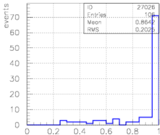
xgamma rejected
